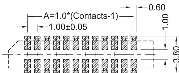
SRX and SVX PCB Layout Reference
