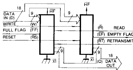
Figure 13. Block Diagram of 2048 \times 18 FIFO Memory Used in Width Expansion Mode
