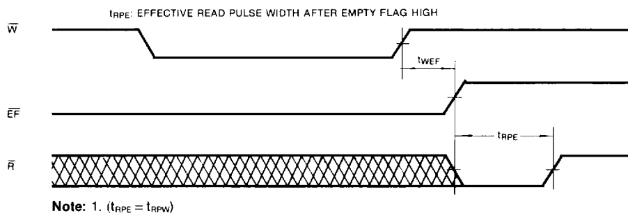
Figure 9. Empty Flag Timing
