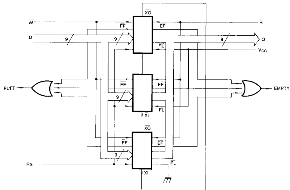
Figure 14. Block Diagram of 1536 × 9 FIFO Memory (Depth Expansion)
