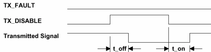
Figure 4 Detection of transmitter fault condition
