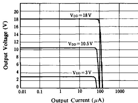
Output Voltage vs. Output Current
