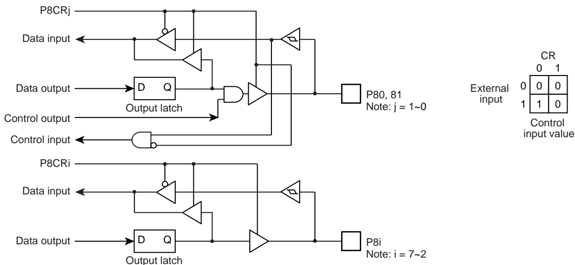
Figure 5-10 Port P8
