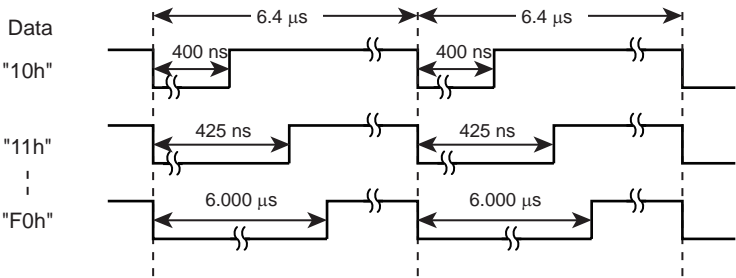
Figure 18-3 7-Bit Mode
