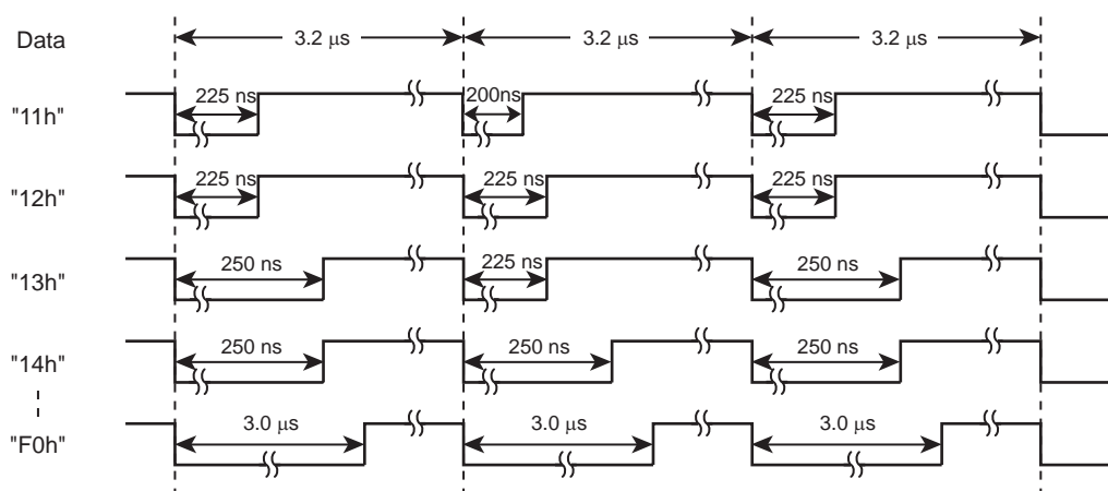
Figure 18-4 6-Bit Mode
