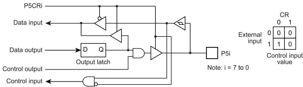
Figure 5-7 Port P5
