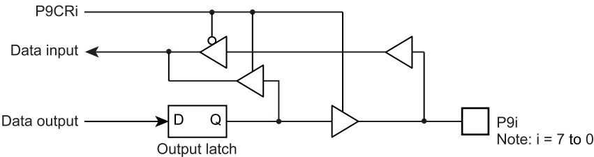
Figure 5-11 Port P9
