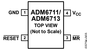
Figure 4. Pin Configuration
