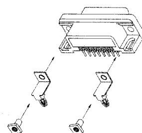
RIVET W/4-PRONG BOARDLOCK
