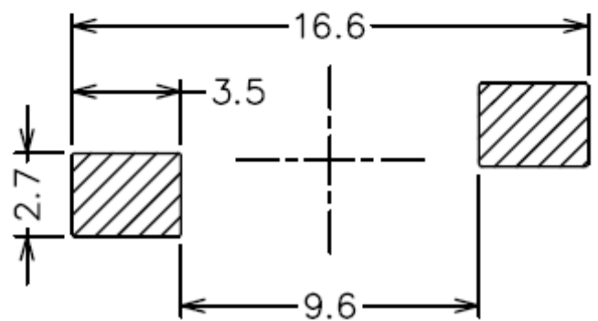
Soldering patterns
