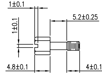
#4-40UNC SCREW
