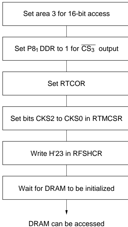
Figure 7-10 Setup Procedure for \overline{2WE} 4-Mbit DRAM with 10-Bit Row Address and 8-Bit Column Address (16-Mbyte Mode)
