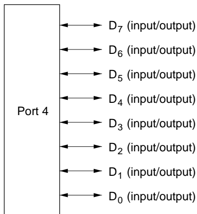
Figure 9-3 Pin Functions in 16-Bit Bus Mode (Port 4)
