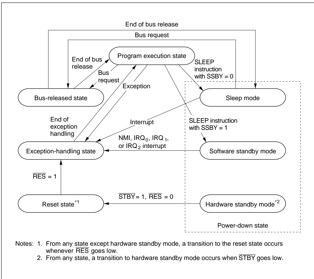
Figure 2-13 State Transitions
