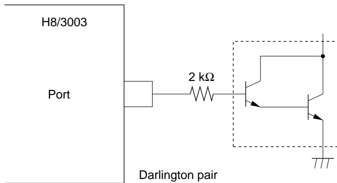
Figure 18-1 Darlington Pair Drive Circuit (Example)
