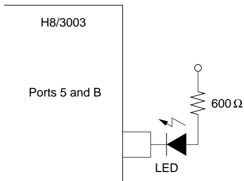
Figure 18-2 LED Drive Circuit (Example)
