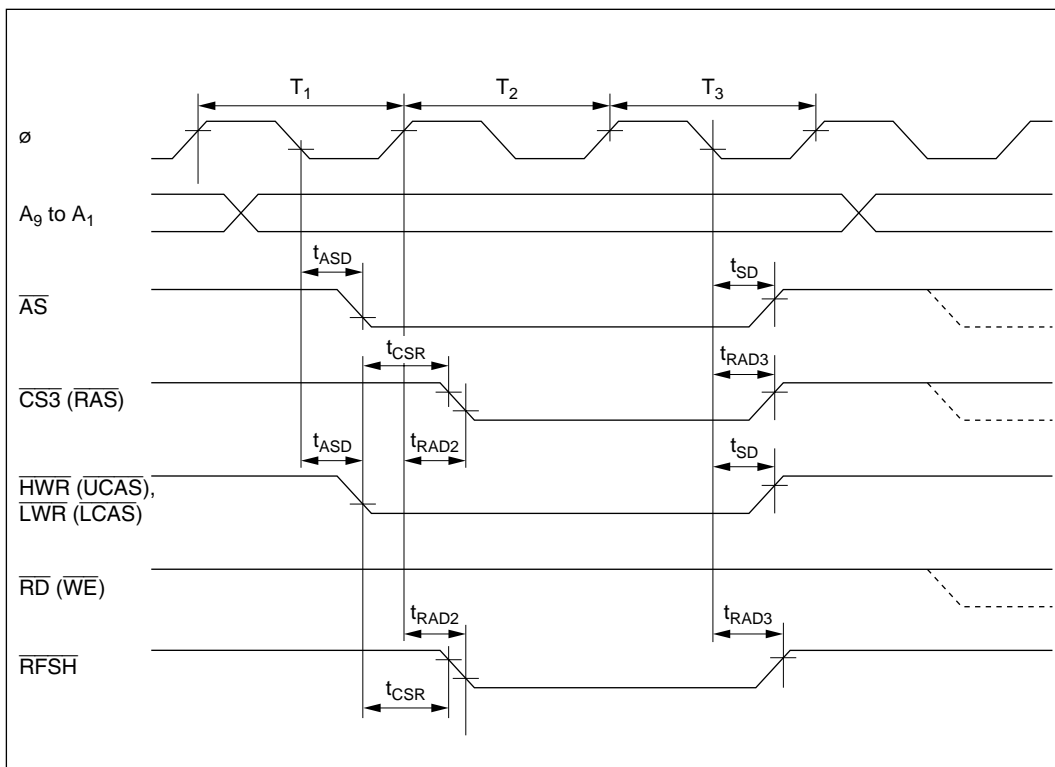
Figure 18-11 DRAM Bus Timing (Refresh Cycle): Three-State Access — 2\overline{\text{CAS}} Mode —
