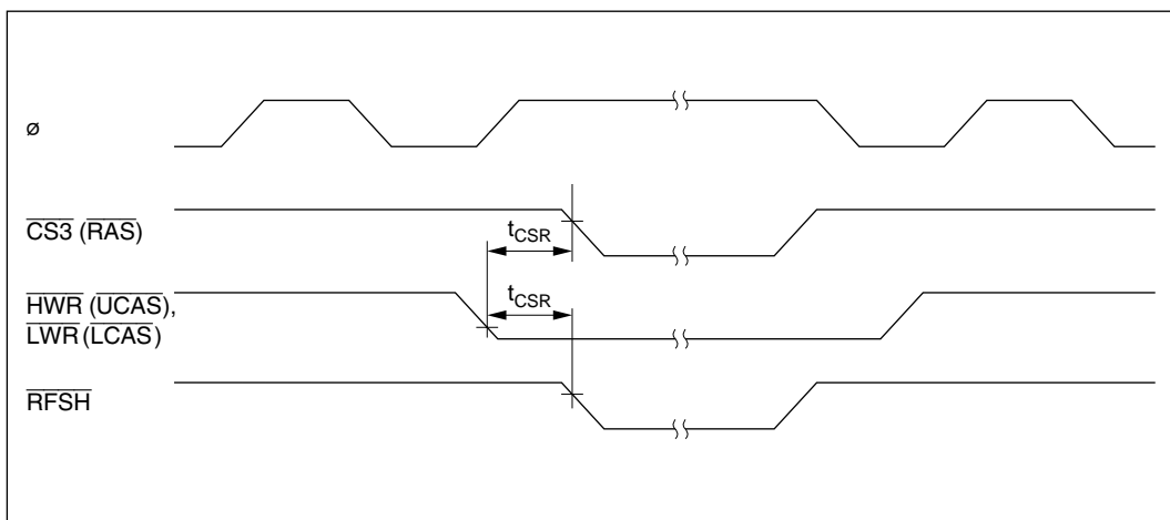
Figure 18-12 DRAM Bus Timing (Self-Refresh Mode) — 2\overline{\text{CAS}} Mode —
