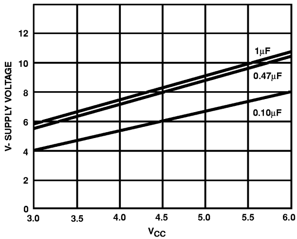
FIGURE 5. V- SUPPLY VOLTAGE vs V_{CC} , VARYING CAPACITORS
