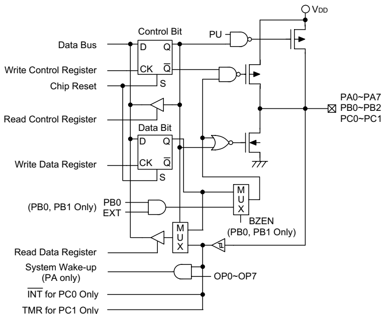
Input/Output Ports
