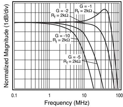
Inverting Freq. Response V_s = +5V
