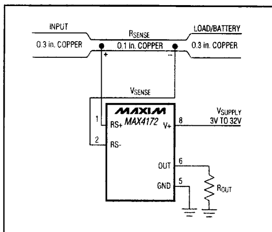
Figure 2. MAX4172 Connections Showing Use of PC Board
