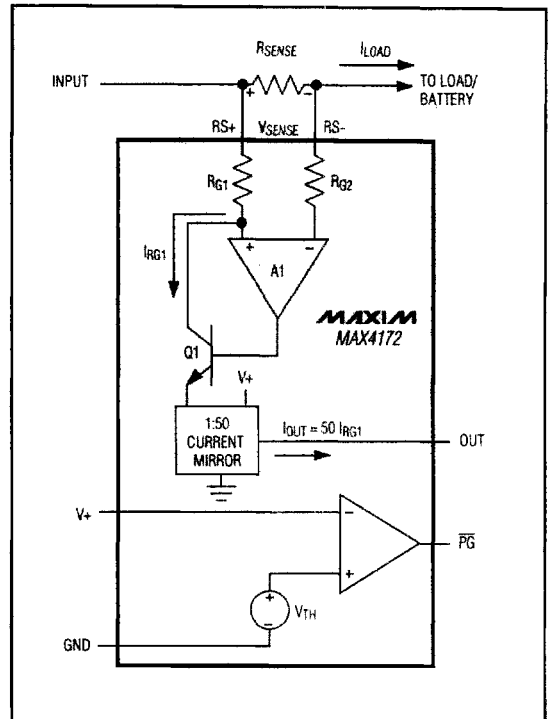
Figure 1. Functional Diagram
