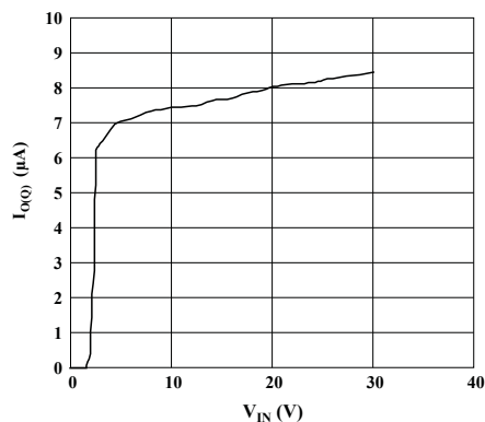
Quiescent Current versus Input Voltage V_{EN} = 0\text{V}
