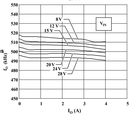
Operating Frequency versus Input Voltage
