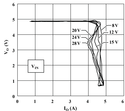
Overcurrent Protection
