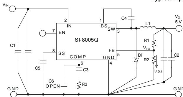
Figure 1. Typical application circuit for general use
