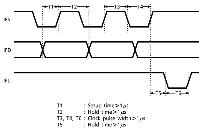
Fig.6 \mu\text{-COM} I/F Timing
