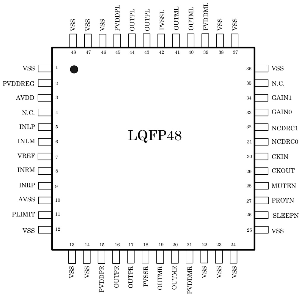
< 48-pin LQFP Top View >
