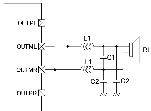
LC Filter circuit (Monaural)
