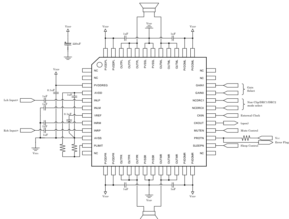
Single operation in stereo mode (single-ended input, external clock operation)
