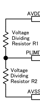
PLIMIT terminal setting circuit
