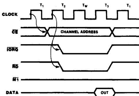
Figure 5. Read Cycle
