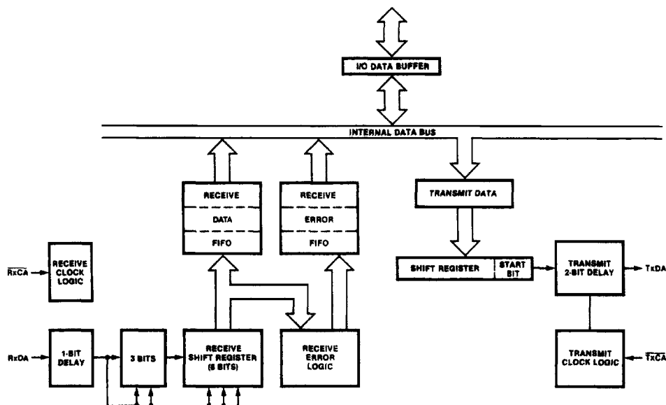
Figure 4. Data Path
