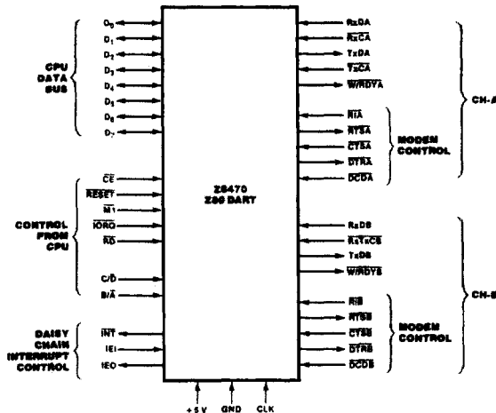
Figure 1. Pin Functions
