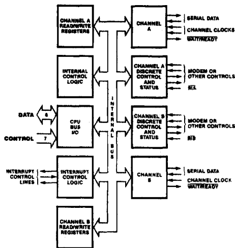
Figure 3. Block Diagram
