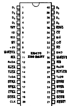
Figure 2. 40-Pin Dual-In-Line Package (DIP), Pin Assignments
