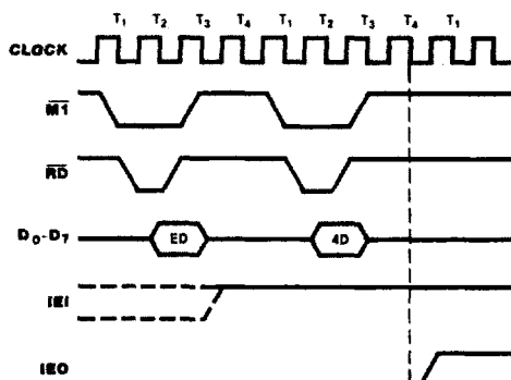
Figure 8. Return from Interrupt Cycle
