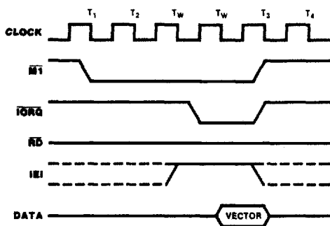
Figure 7. Interrupt Acknowledge Cycle
