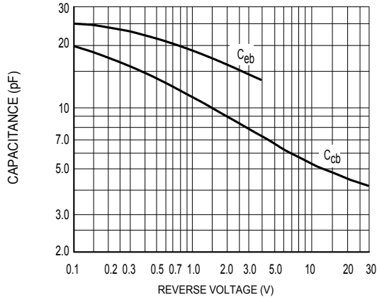
Figure 1. Capacitances
