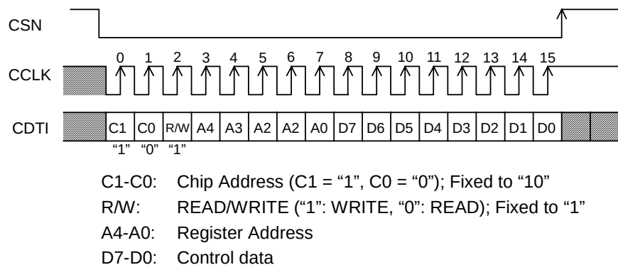
Figure 35. Serial Control I/F Timing
