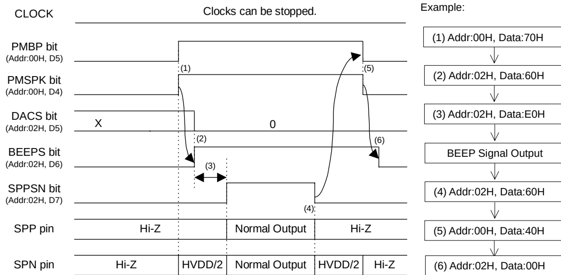
Figure 52. “BEEP-Amp → Speaker-Amp” Output Sequence
