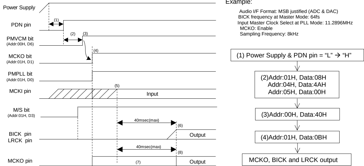
Figure 46. Clock Set Up Sequence (1)
