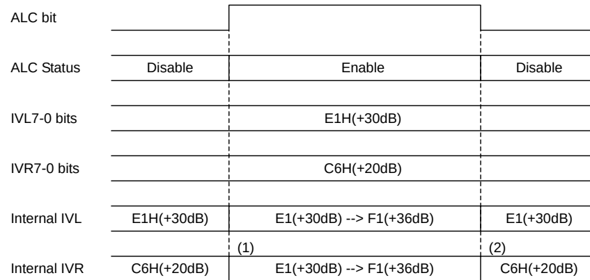
Figure 25. IVOL value during ALC operation
