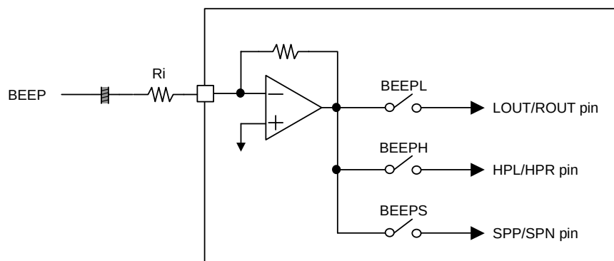
Figure 7. Block Diagram of BEEP pin
