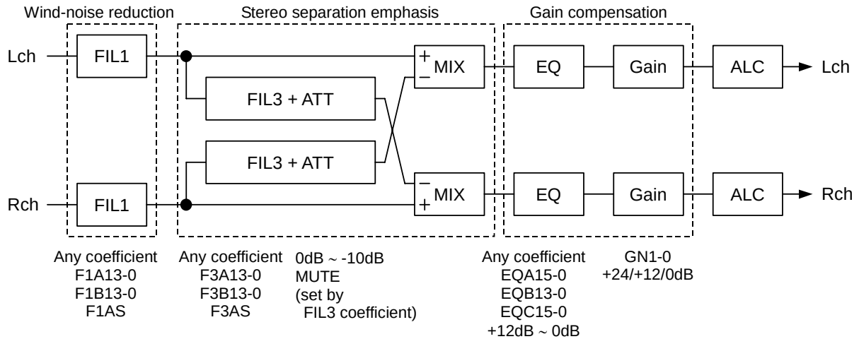
Figure 23. Digital EQ/HPF/LPF
