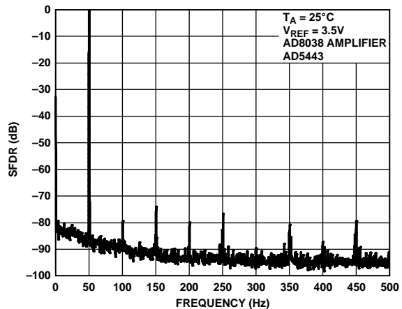
Figure 35. Wideband SFDR f_{OUT} = 50 kHz, Update = 1 MHz
