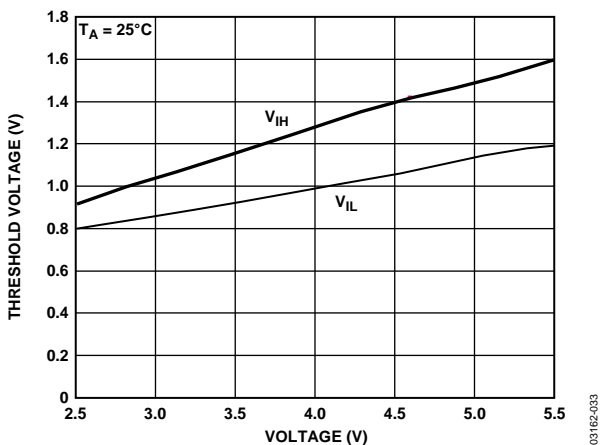
Figure 32. Threshold Voltages vs. Supply Voltage
