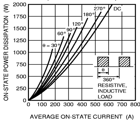
MAXIMUM ON-STATE POWER DISSIPATION CHARACTERISTICS (RECTANGULAR WAVE)
