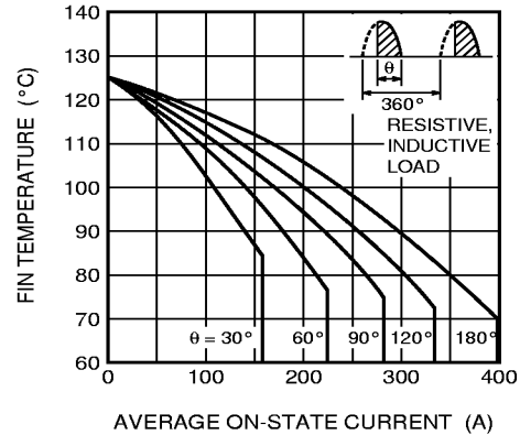
ALLOWABLE FIN TEMPERATURE VS. AVERAGE ON-STATE CURRENT (SINGLE-PHASE HALF WAVE)
