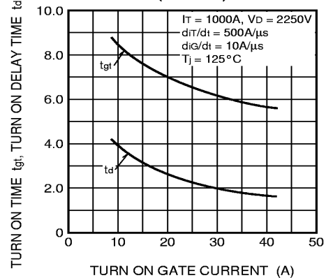
TURN ON TIME, TURN ON DELAY TIME VS. TURN ON GATE CURRENT (TYPICAL)
