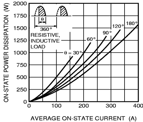
MAXIMUM ON-STATE POWER DISSIPATION CHARACTERISTICS (SINGLE-PHASE HALF WAVE)
