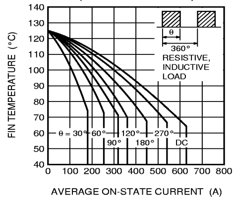
ALLOWABLE FIN TEMPERATURE VS. AVERAGE ON-STATE CURRENT (RECTANGULAR WAVE)
