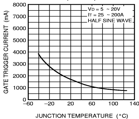
GATE TRIGGER CURRENT VS. JUNCTION TEMPERATURE (TYPICAL)
