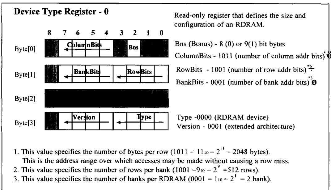
Figure 13. Registers
