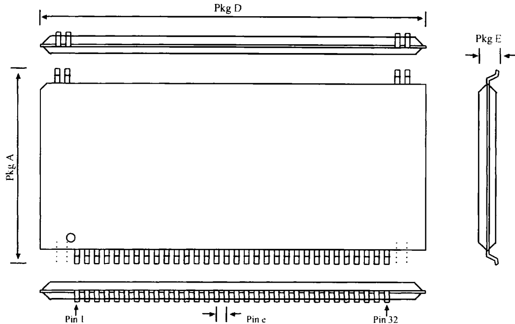
FIGURE 31. SHP-32 Package
