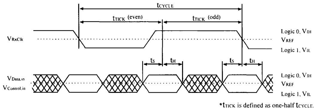
FIGURE 16. Receive Data Timing
