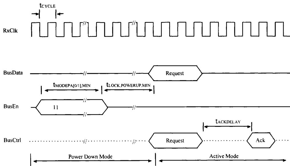
FIGURE 30. Power Up Timing
