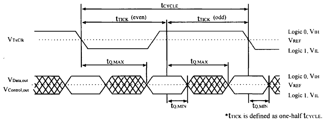
FIGURE 17. Transmit Data Timing
