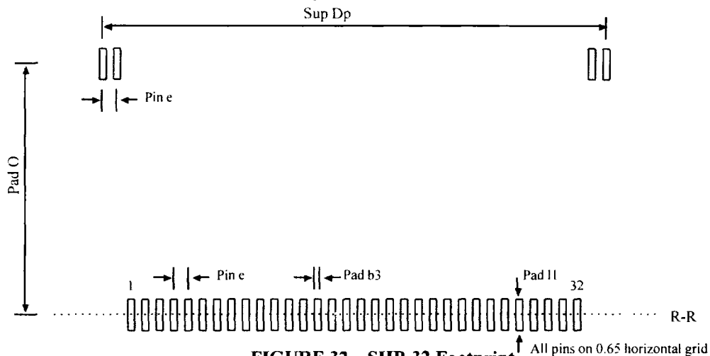
FIGURE 32. SHP-32 Footprint
