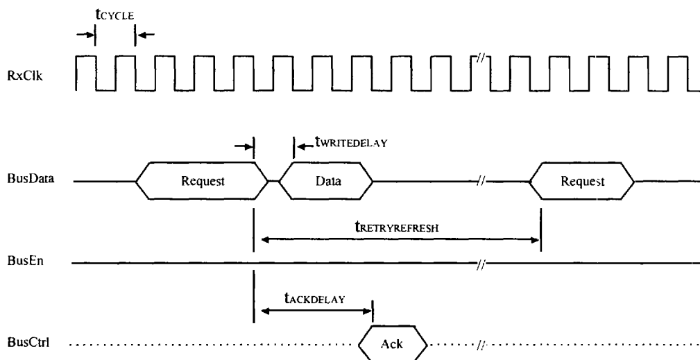
FIGURE 27. Manual Refresh Using SetRR
