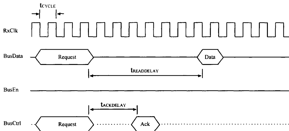
FIGURE 25. Register Read Timing Diagram
