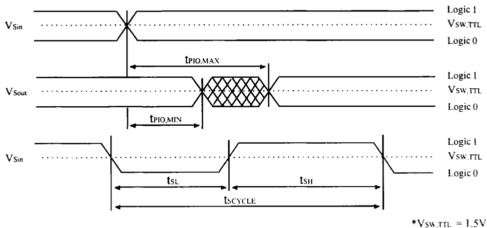
FIGURE 18. Serial Configuration Pin Timing
