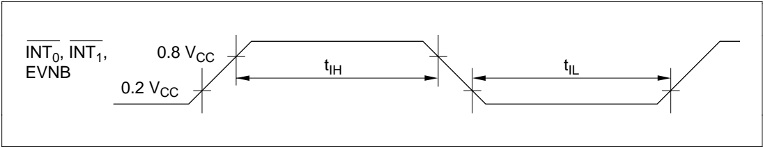
Figure 25-32 Interrupt Timing (HD404369 Series)
