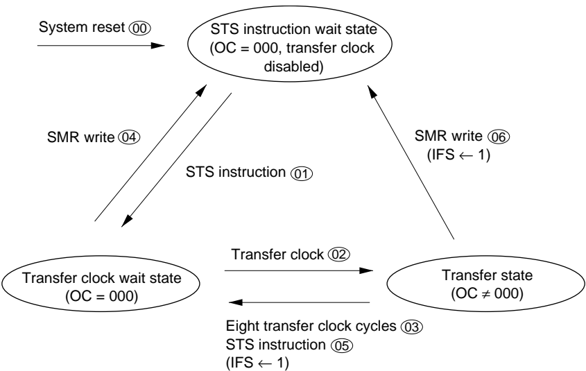
(1) External Clock Mode
