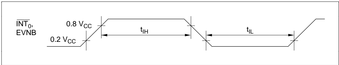
Figure 25-8 Interrupt Timing (HD404394 Series)
