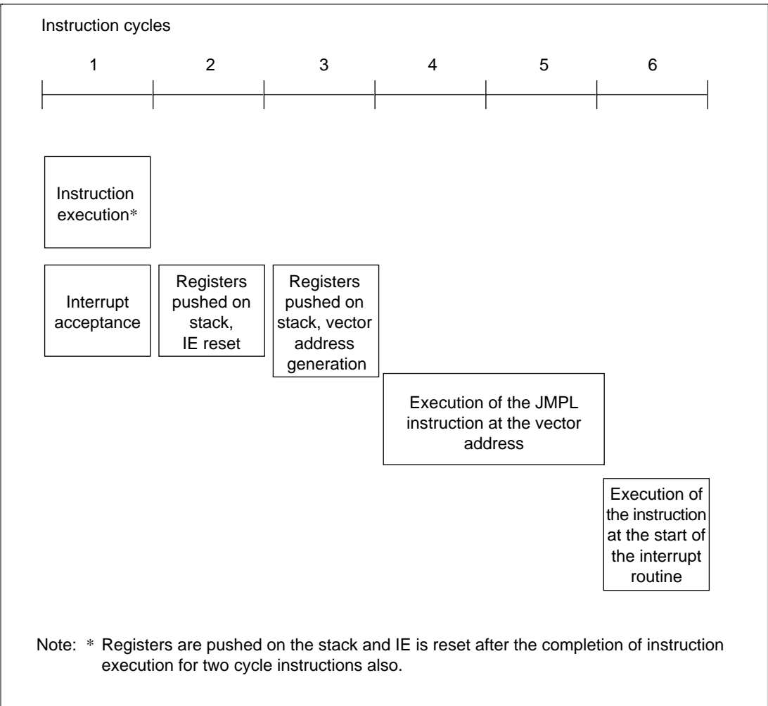
Figure 4-3 Interrupt Handling Sequence
