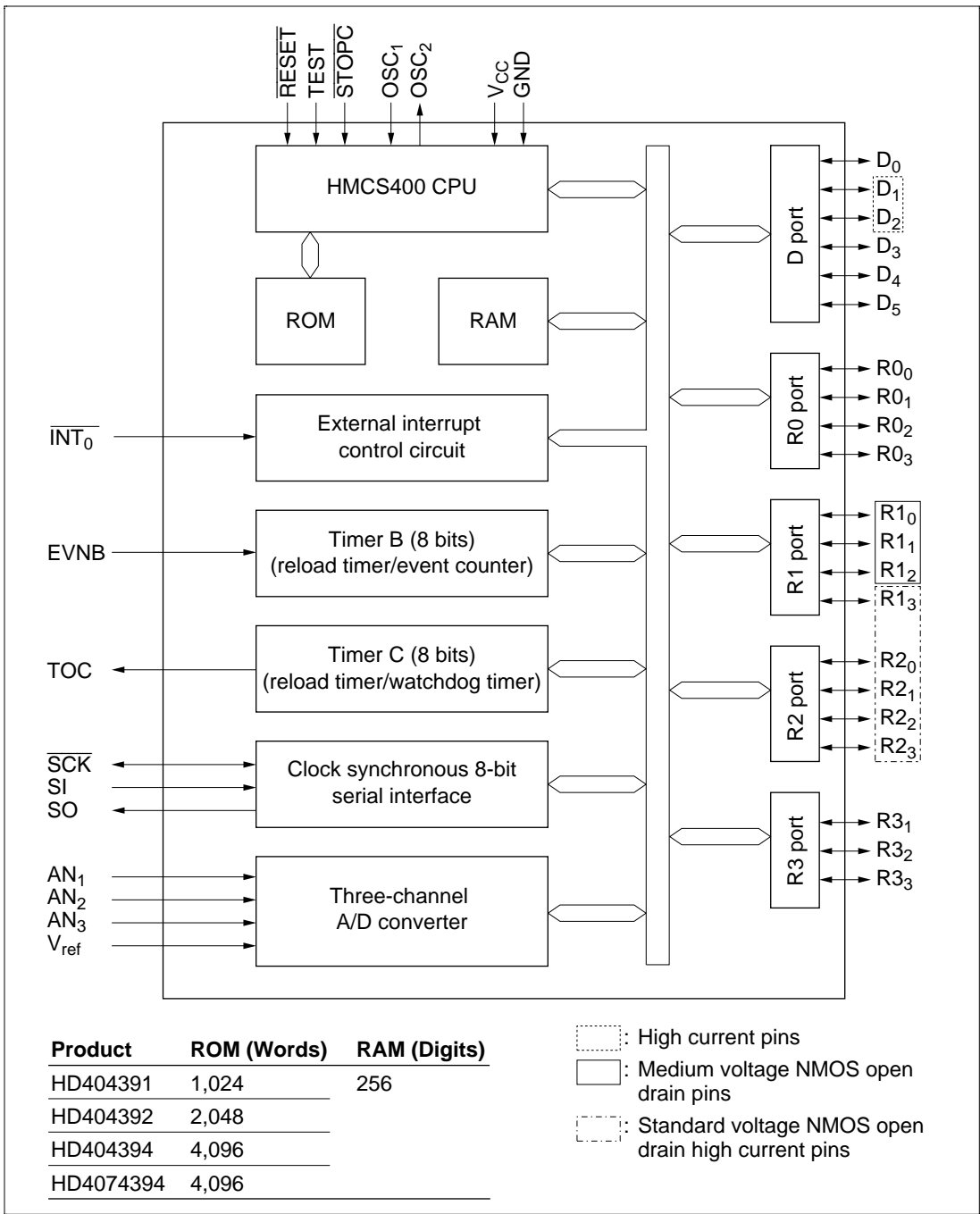
Figure 1-3 HD404394 Series Internal Block Diagram
