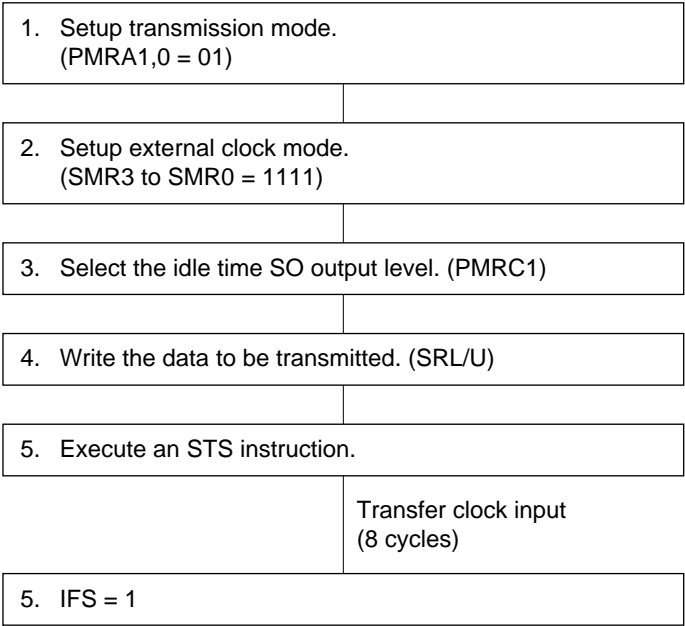
Figure 20-5 Data Transmission Procedure (External Clock Mode)
