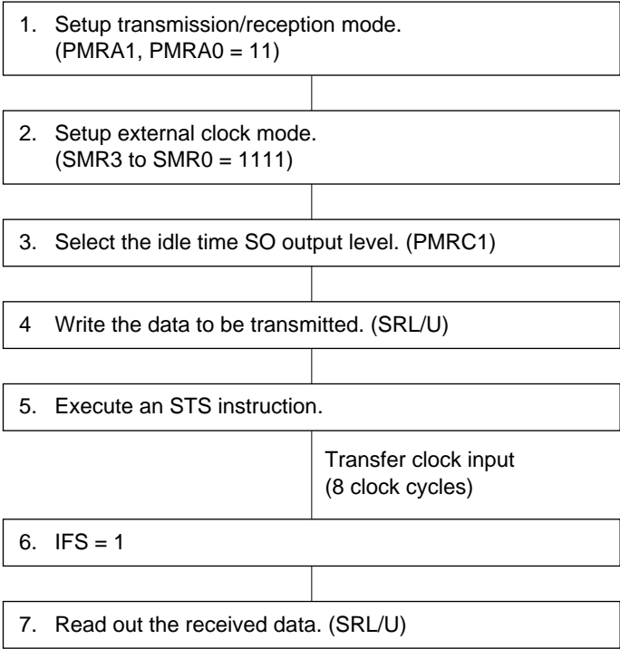
Figure 20-13 Simultaneous Transmission and Reception Procedure (External Clock Mode)
