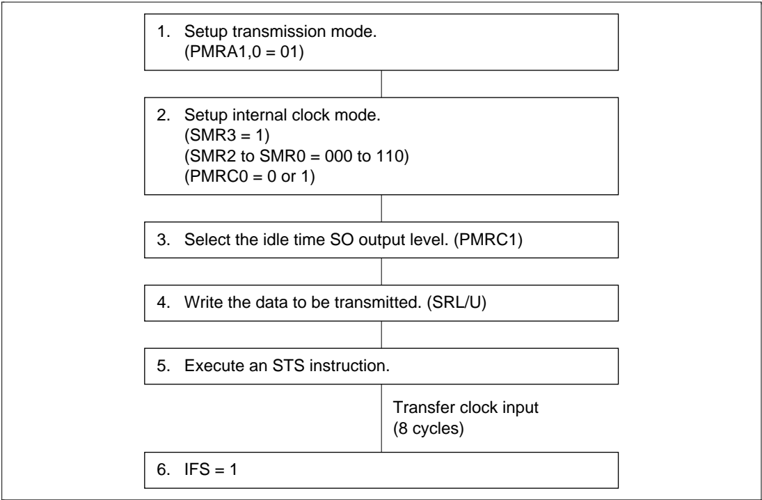
Figure 20-7 Data Transmission Procedure (Internal Clock Mode)
