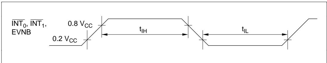
Figure 25-14 Interrupt Timing (HD404318 Series)
