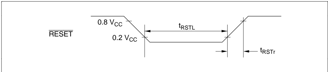
Figure 25-9 Reset Timing (HD404394 Series)
