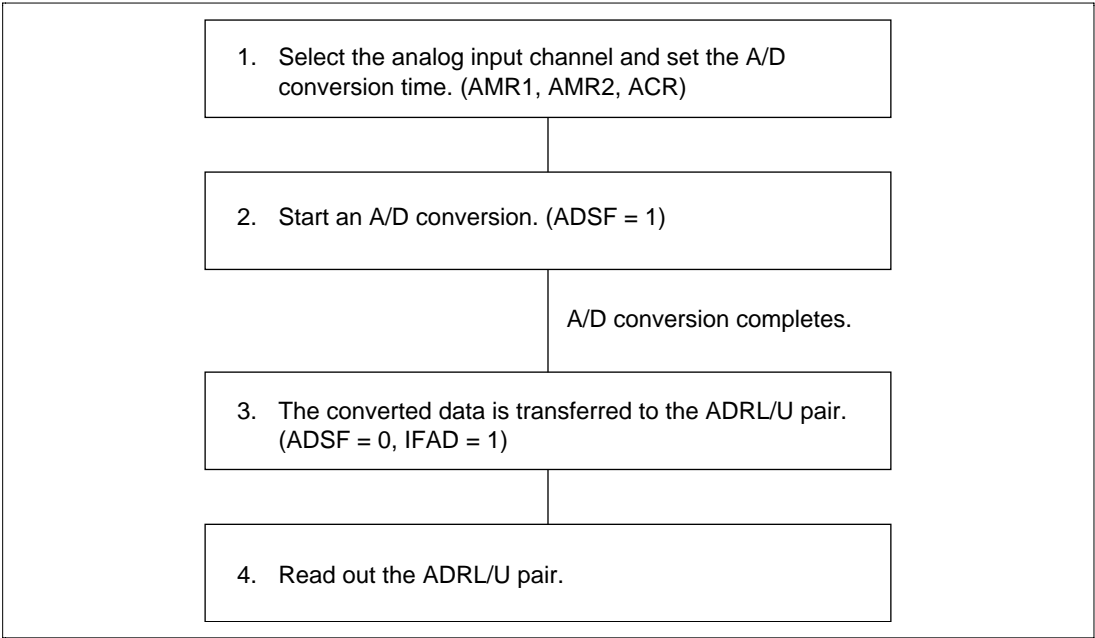
Figure 15-2 A/D Conversion Operation Sequence
