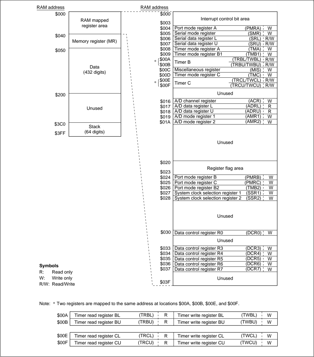
Figure 2-6 HD404339 Series RAM Memory Map
