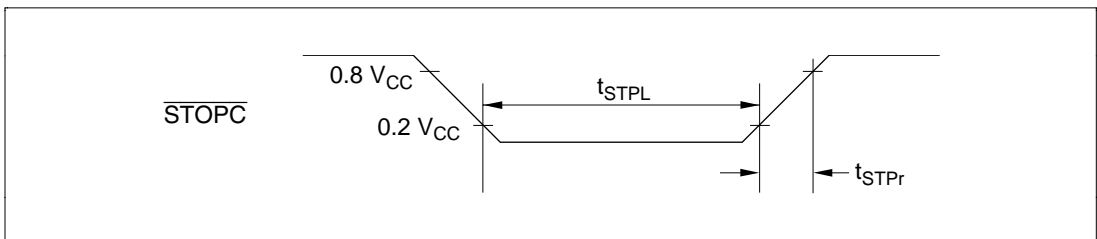
Figure 25-16 \overline{STOPC} Timing (HD404318 Series)
