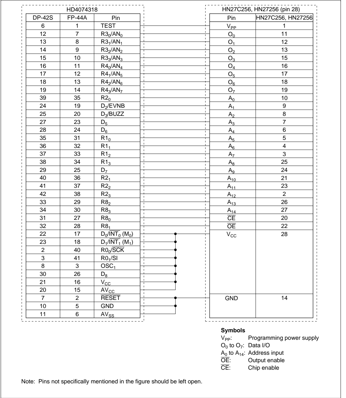
Figure 22-2 HD4074318 Socket Adapter Pin Correspondence
