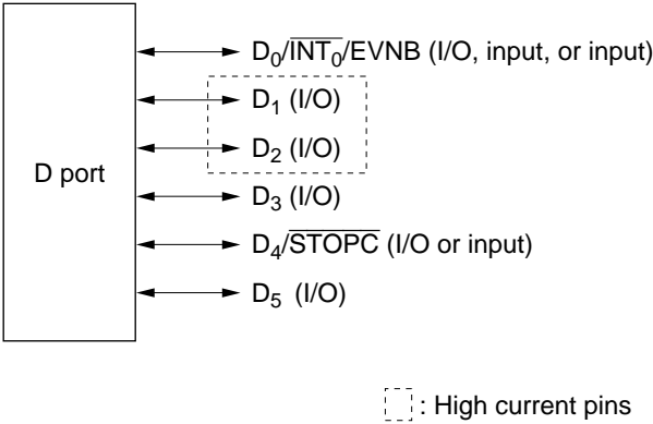
Figure 8-1 D Port Structure
