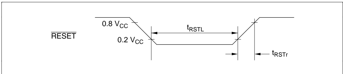
Figure 25-15 Reset Timing (HD404318 Series)
