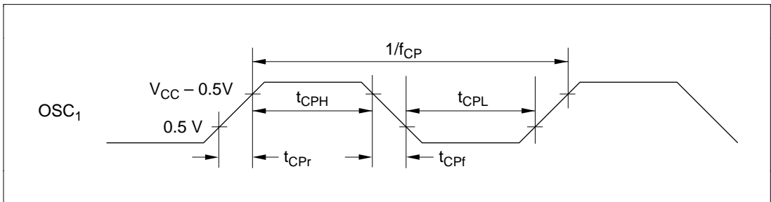
Figure 25-13 External Clock Timing (HD404318 Series)
