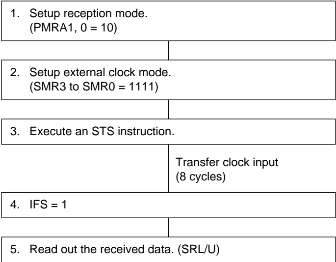
Figure 20-9 Data Reception Procedure (External Clock Mode)
