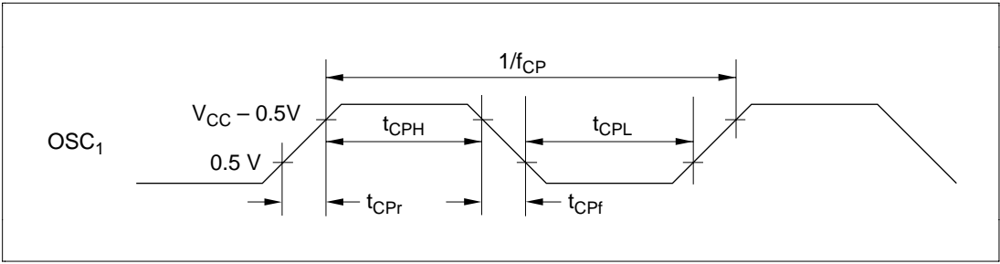
Figure 25-31 External Clock Timing (HD404369 Series)
