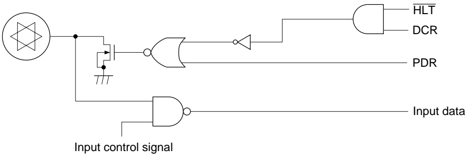
(b) ZTAT TM and Mask ROM Pin Circuit Structure
