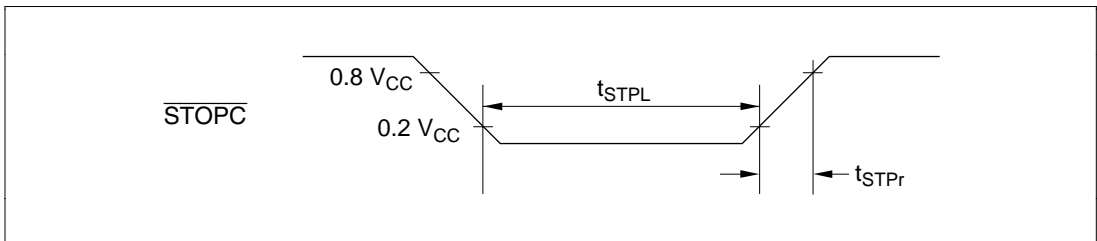
Figure 25-10 STOPC Timing (HD404394 Series)
