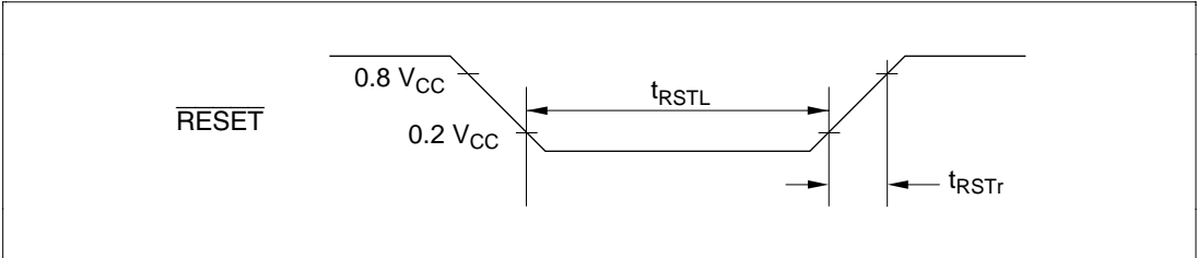
Figure 25-33 Reset Timing (HD404369 Series)
