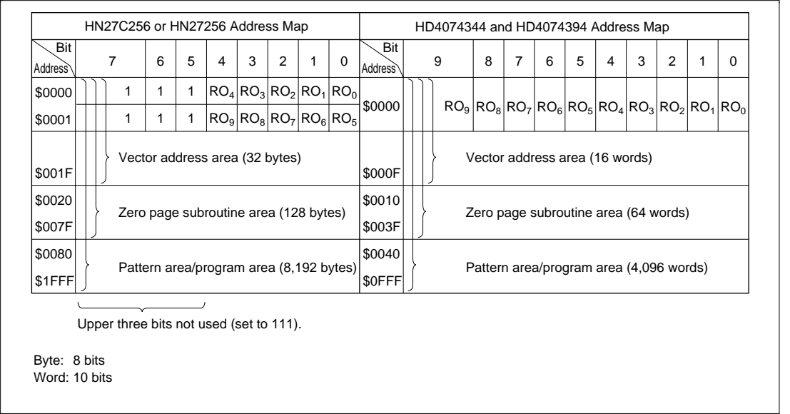
Figure 22-6 HD4074344 and HD4074394 PROM Mode Memory Map
