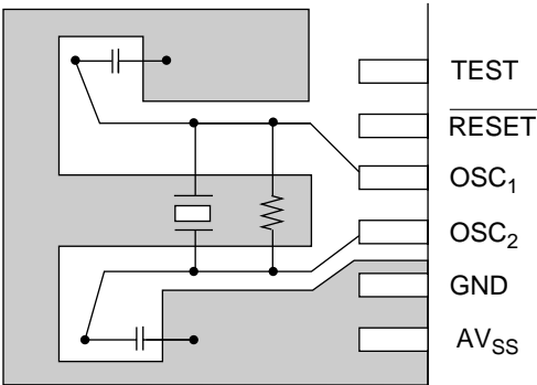
Figure 13-2 Wiring Examples for Crystal and Ceramic Oscillators
