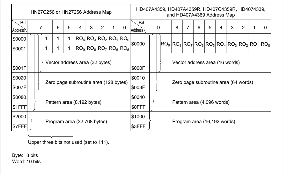
Figure 22-8 HD407A4359, HD407A4359R, HD407C4359R, HD4074339, and HD407A4369 PROM Mode Memory Map
