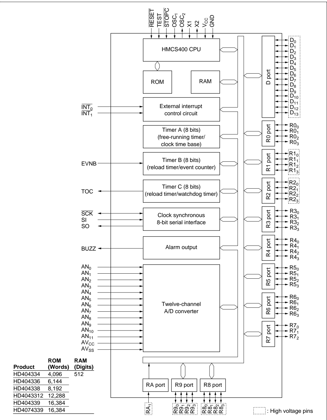
Figure 1-7 HD404339 Series Internal Block Diagram
