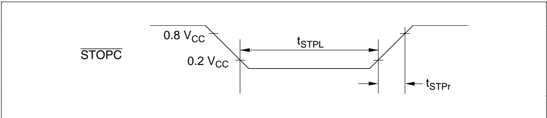
Figure 25-34 STOPC Timing (HD404369 Series)
