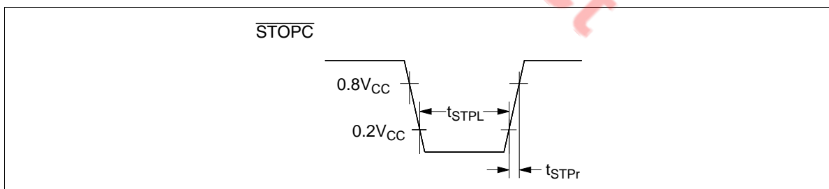
Figure 69 STOPC Timing
