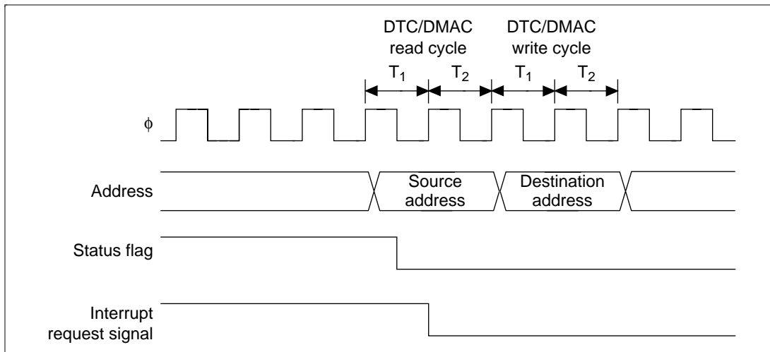
Figure 12.76 Timing of Status Flag Clearing by DTC/DMAC Activation
