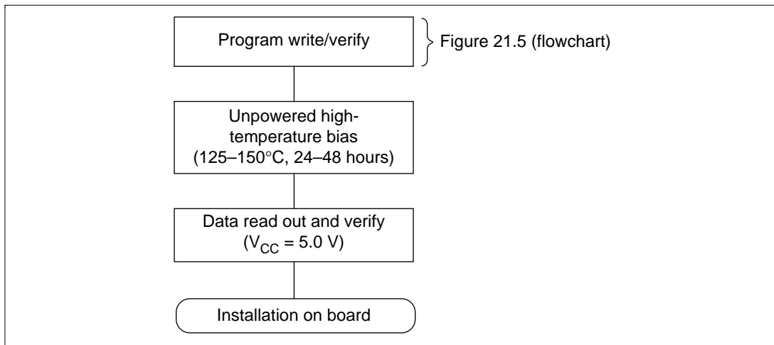
Figure 21.7 Screening Flow
