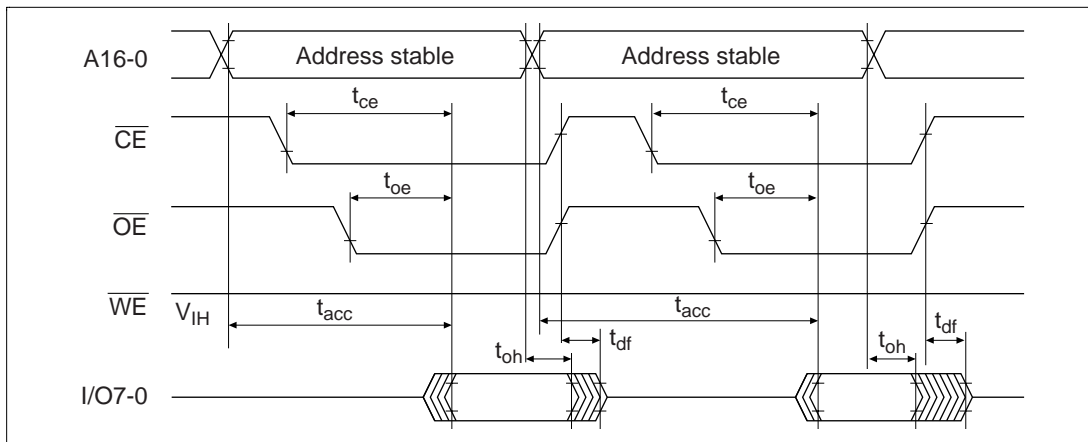
Figure 22.18 \overline{\text{CE}} and \overline{\text{OE}} Clock System Read Timing Waveforms
