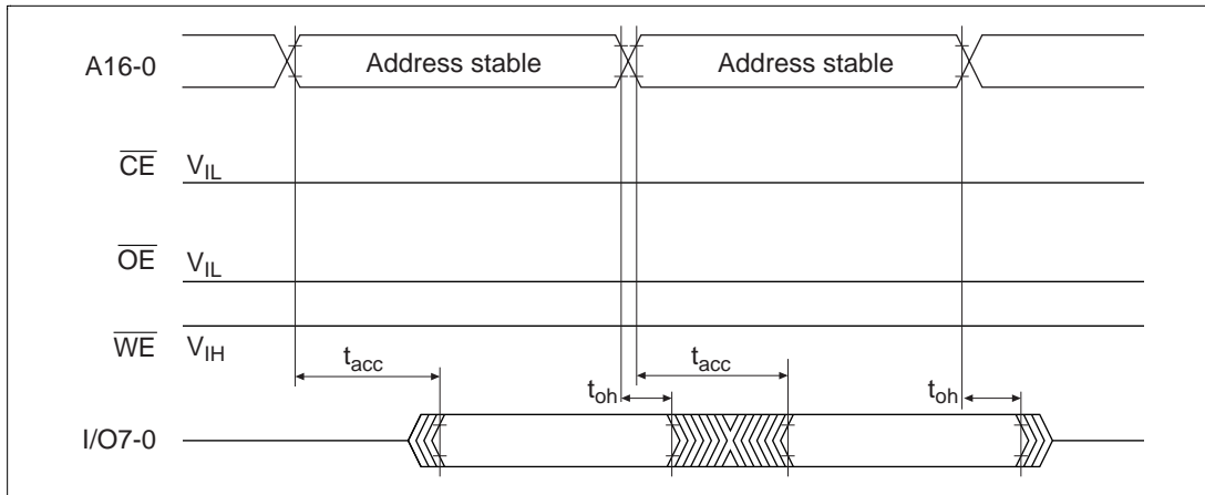
Figure 22.17 \overline{\text{CE}} and \overline{\text{OE}} Enable State Read Timing Waveforms
