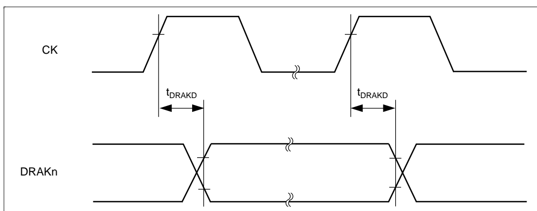
Figure 27.22 DRAKn Output Delay Time
