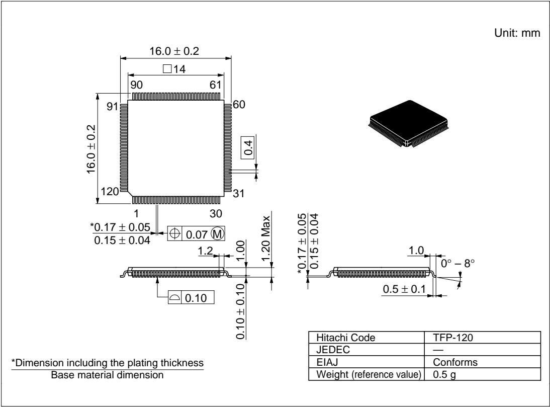
Figure D.2 Package Dimensions (TFP-120)
