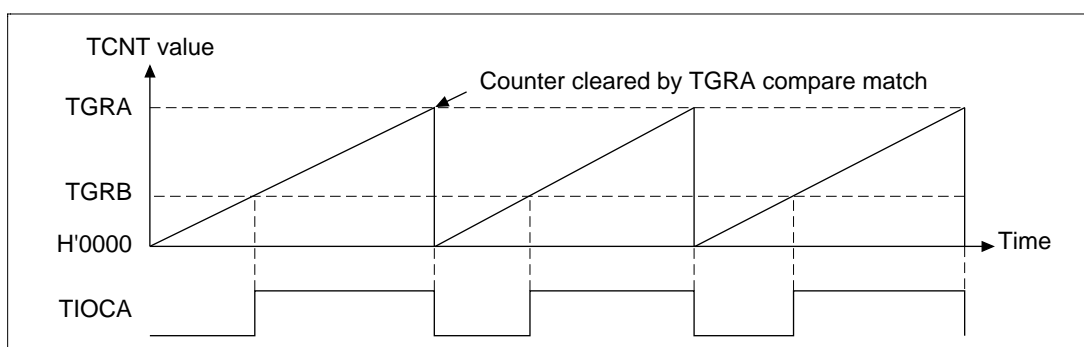
Figure 12.26 PWM Mode Operation Example (Mode 1)
