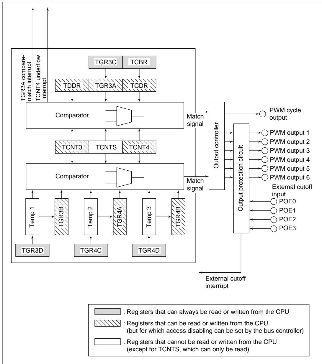
Figure 12.38 Block Diagram of Channels 3 and 4 in Complementary PWM Mode
