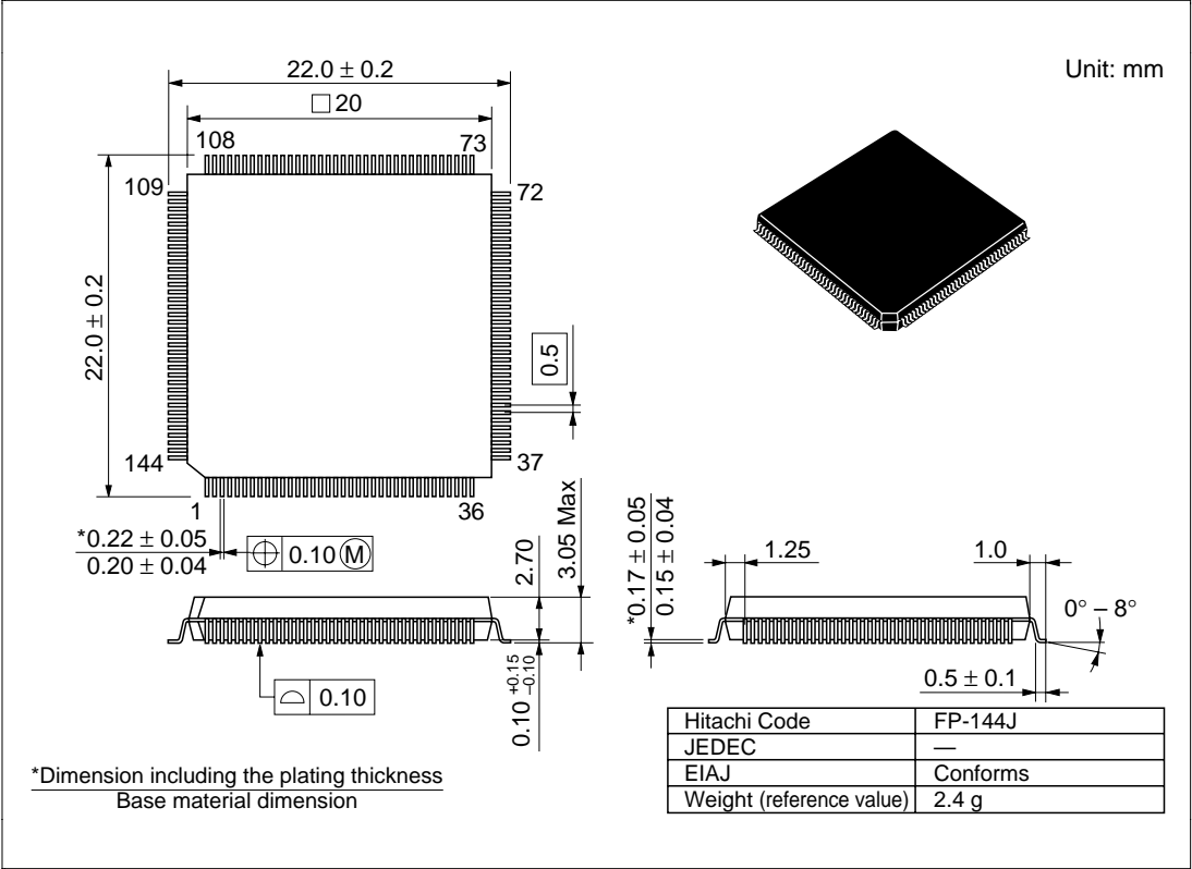
Figure D.3 Package Dimensions (FP-144J)
