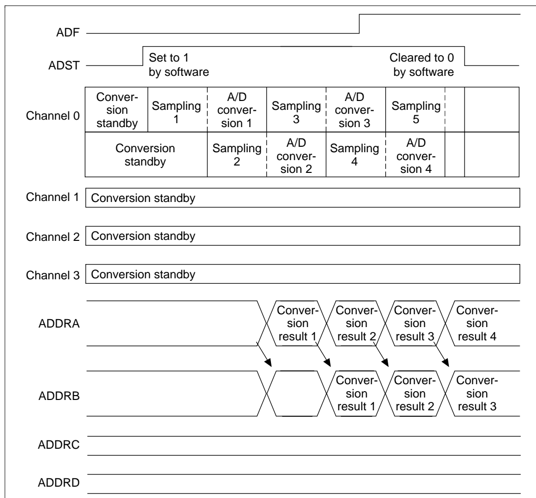
Figure 15.7 Buffer Operation Example (Select Scan Mode: Two-Stage One-Group Operation, When CH2-CH0 = B'001)
