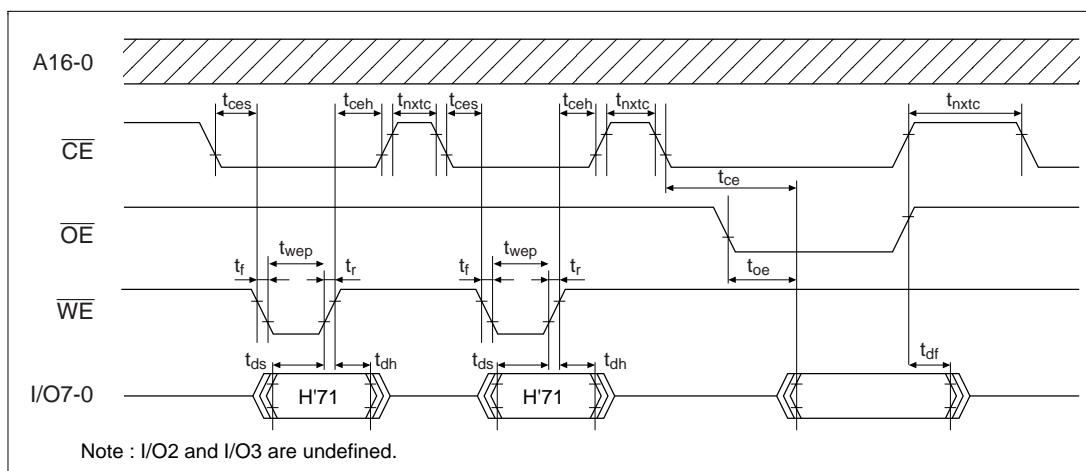
Figure 22.21 Status Read Mode Timing Waveforms
