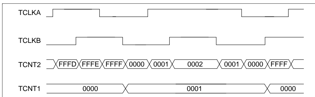
Figure 12.24 Cascade Connection Operation Example (Phase Counting Mode)
