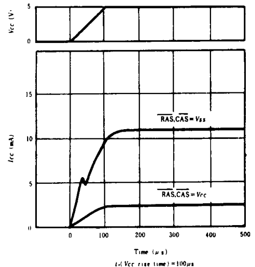
Fig.1 I_{CC} vs. V_{CC} during power up.
