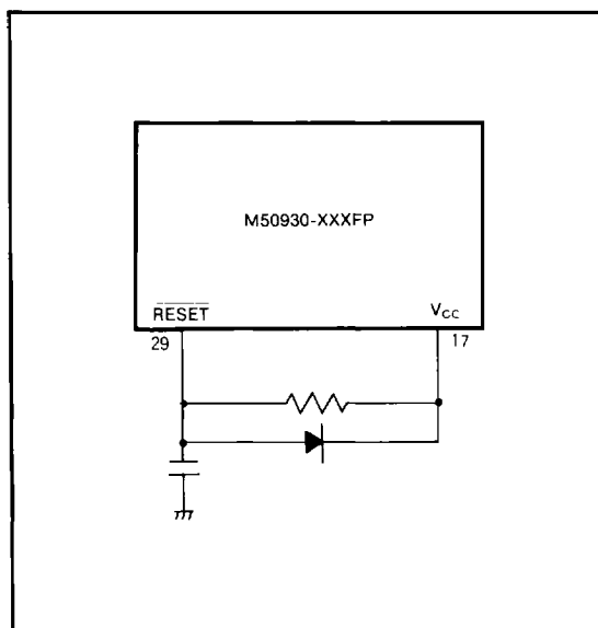
Fig.19 Example of reset circuit
