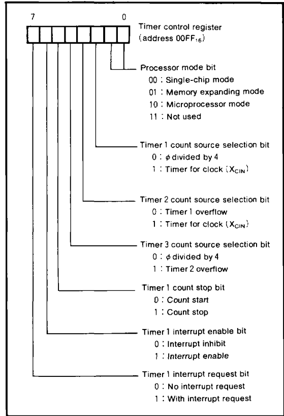
Fig.4 Structure of timer control register
