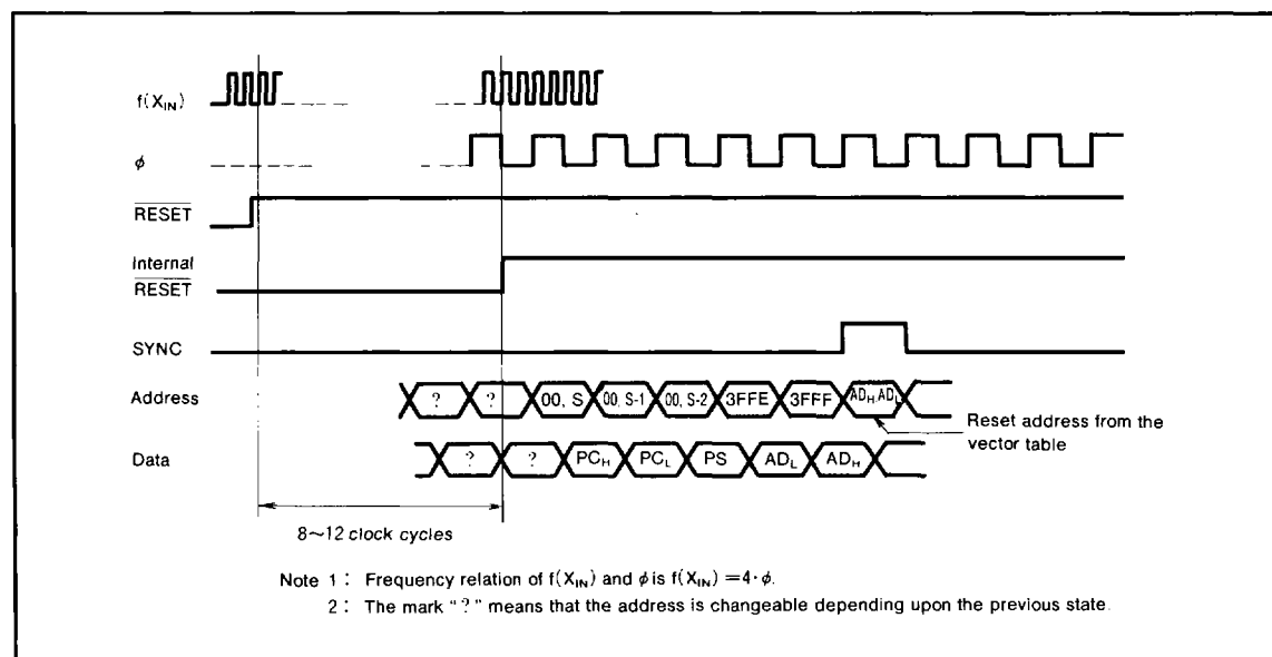
Fig.20 Timing diagram at reset
