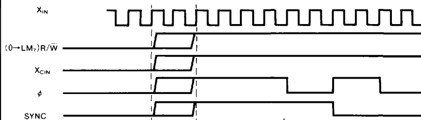
Fig.29 Timing diagram of the changing system clock
