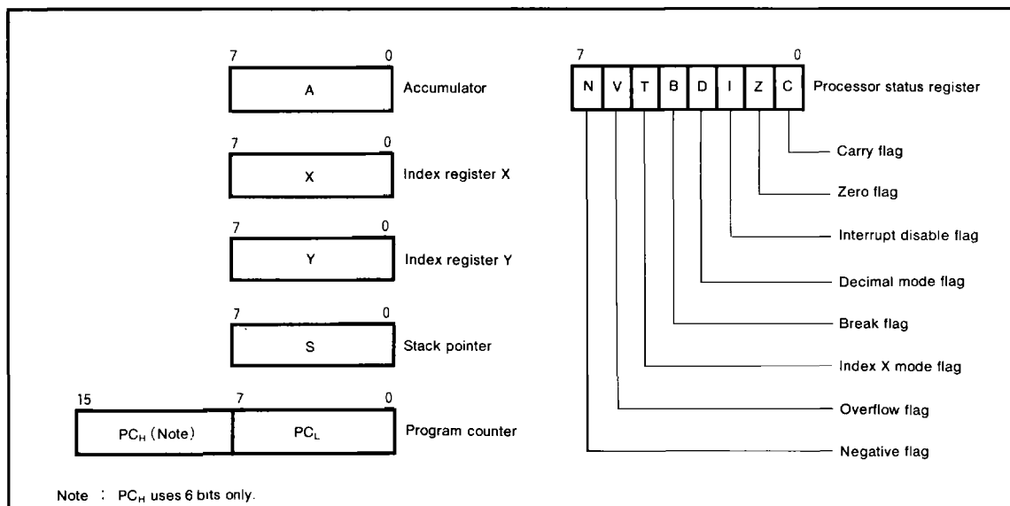
Fig.2 Register structure
