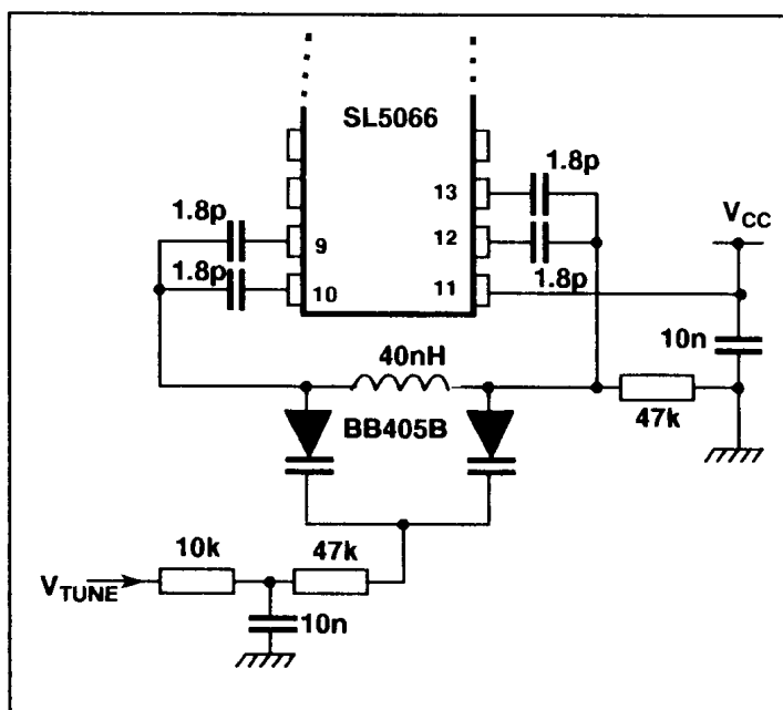
Fig.8 Test circuit
