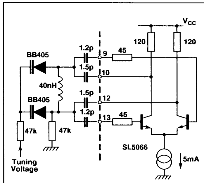
Fig.7 RF oscillator
