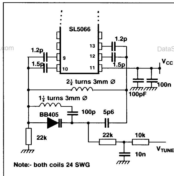
Fig.9 UHF application
