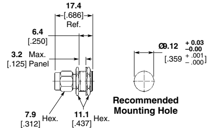
Part No. 1059758-1
