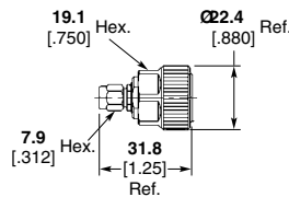
Part No. 1053646-1
