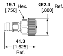
Part No. 1061758-1
