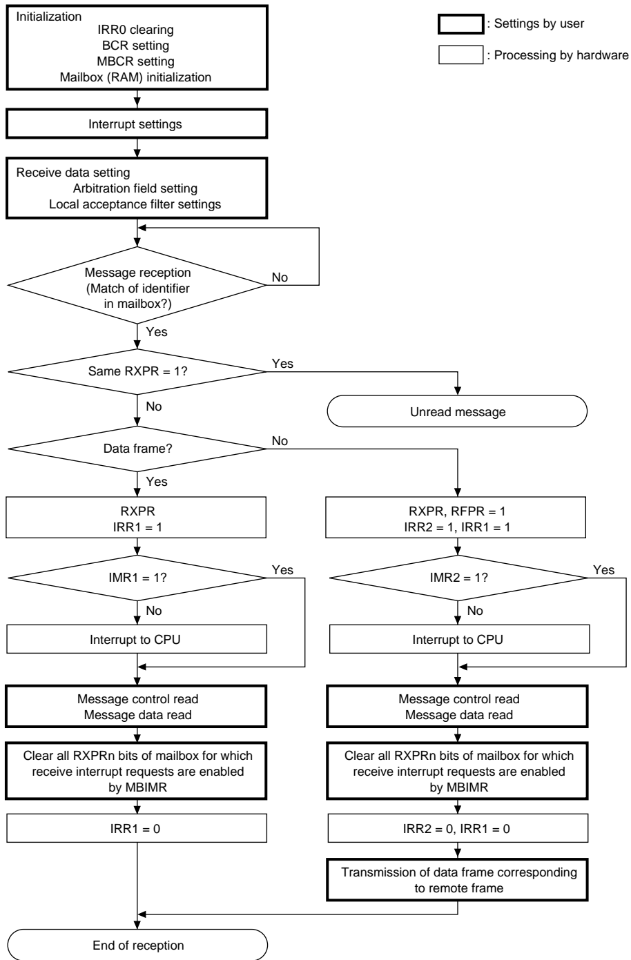
Figure 16-9 Reception Flowchart
