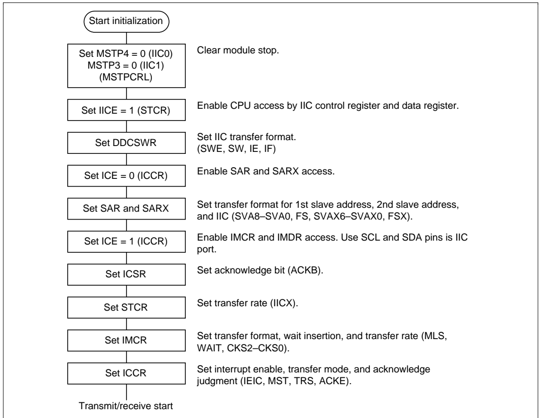
Figure 15-6 Flowchart for IIC Initialization (Example)
