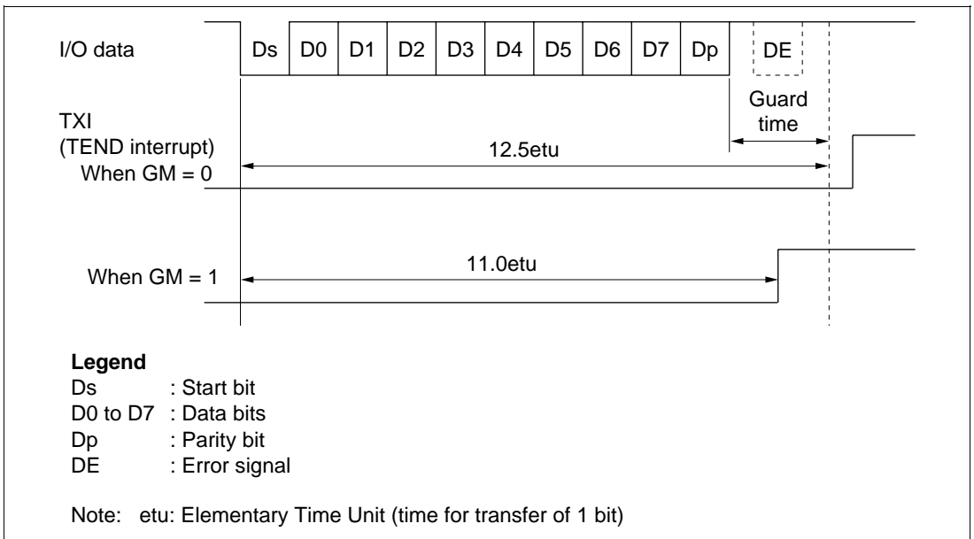
Figure 14-6 TEND Flag Generation Timing in Transmission Operation
