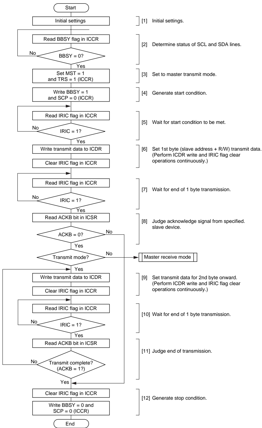
Figur45-7 Flowchart for Master Transmit Mode (Example)
