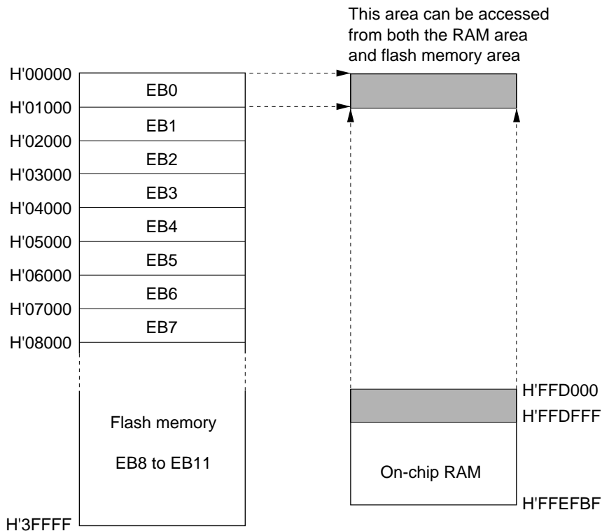
Figure 21B-16 Example of RAM Overlap Operation
