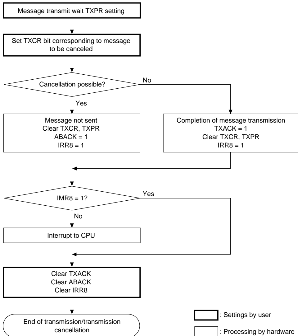
Figure 16-8 Transmit Message Cancellation Flowchart
