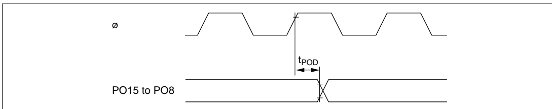
Figure 24-18 PPG Output Timing
