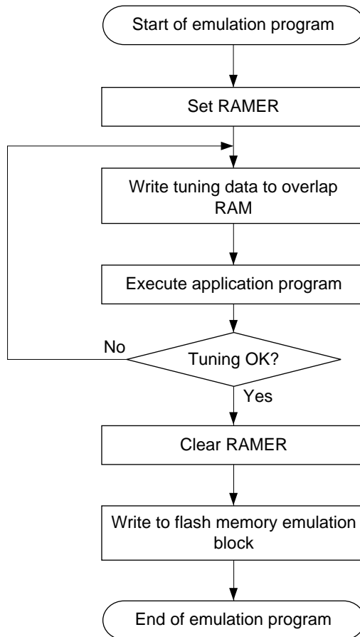
Figure 21A-15 Flowchart for Flash Memory Emulation in RAM
