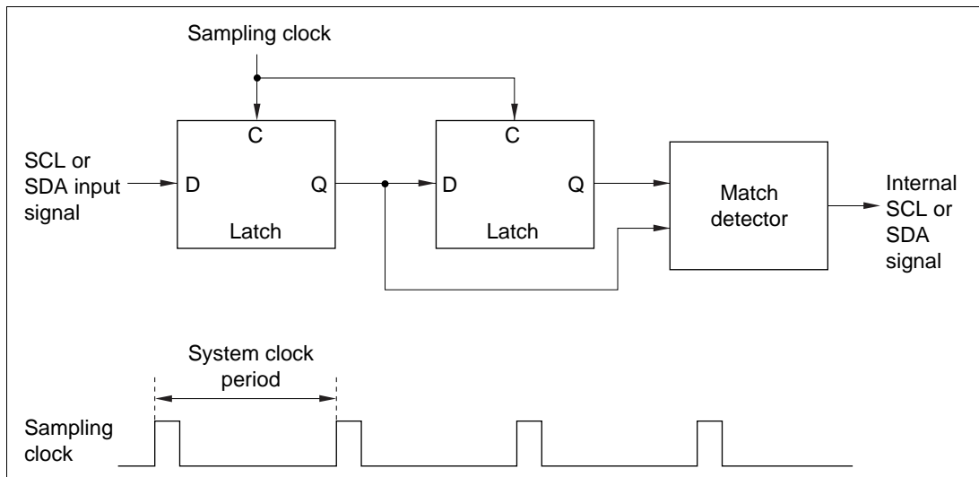
Figure 15-18 Block Diagram of Noise Canceler
