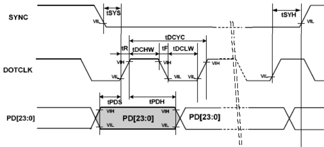
AC Characteristics
