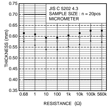
Fig.4 Dimensions (thickness)
