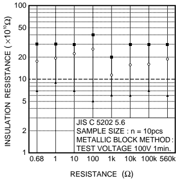
Fig.8 Insulation resistance
