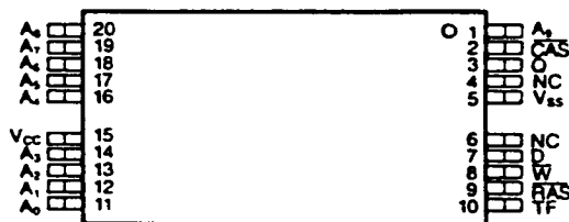
Figure 5. TSOP II (Reverse)
