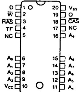
Figure 2. SOJ Package
