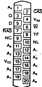
Figure 3. ZIP Package
