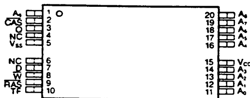
Figure 4. TSOP II (Forward)
