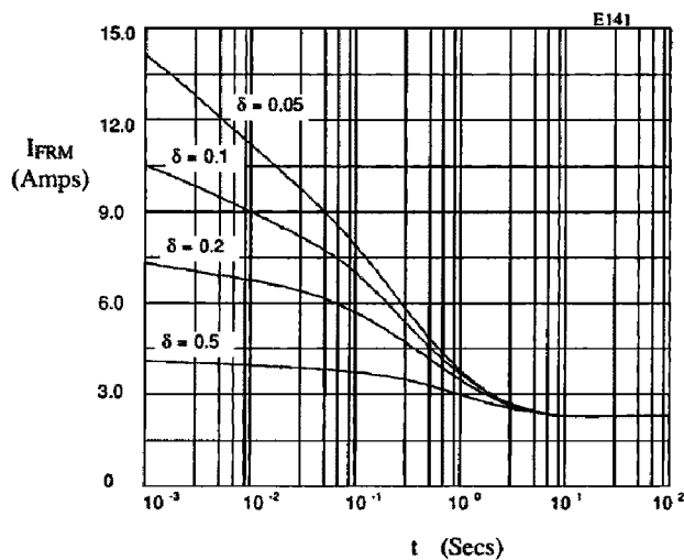
Fig 7. Typical repetitive forward current as a function of pulse width at 55°C; R_{\theta JL} = 45 °C/W; V_{RWM} during 1 - \delta .
