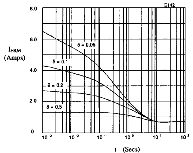
Fig 8. Typical repetitive forward current as a function of pulse width at 100°C; R_{\theta JL} = 100 °C/W; V_{RWM} during 1 - \delta .
