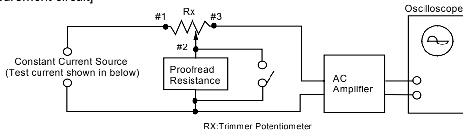
[Measurement circuit]
