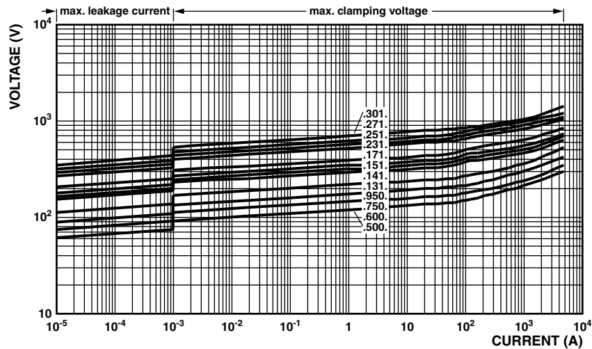
50 V RMS to 300 V RMS ; VDRH14.....E
