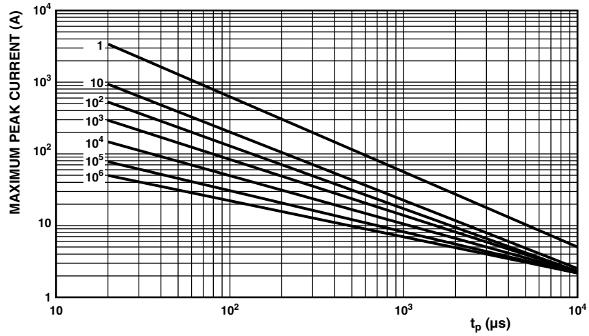
320 V RMS to 680 V RMS ; VDRH10.....E
