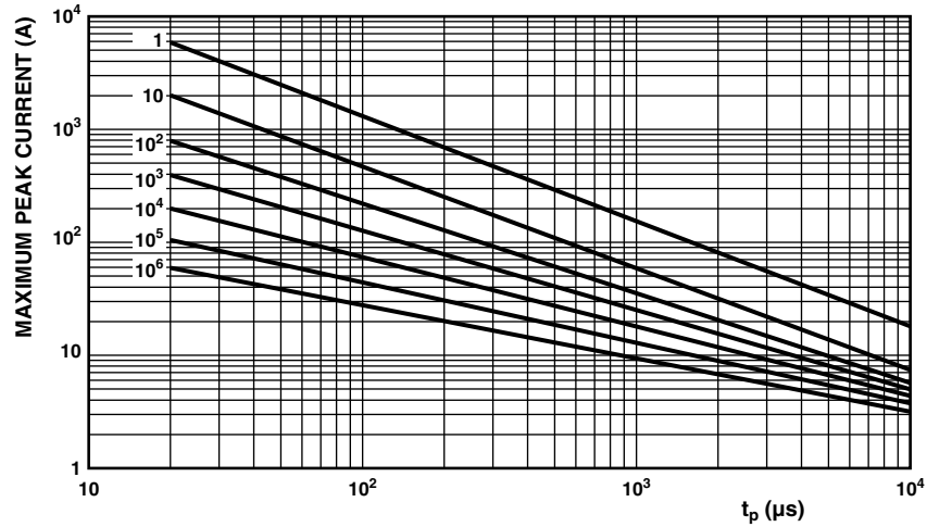
320 V RMS to 680 V RMS ; VDRH14.....E
