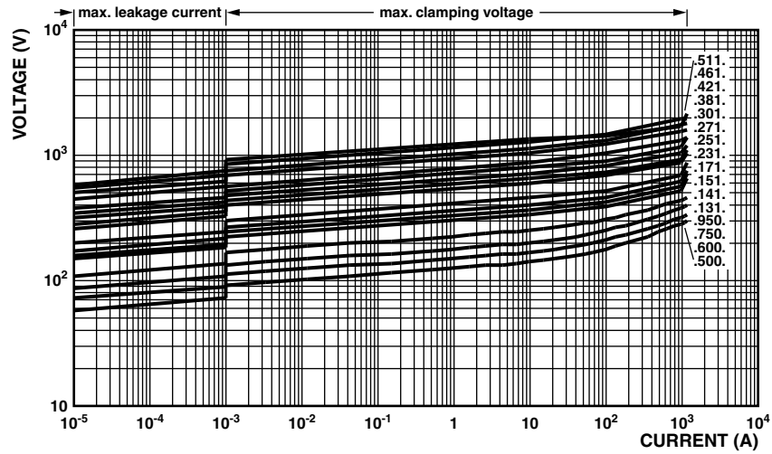
11 V RMS to 40 V RMS ; VDRH10.....E
