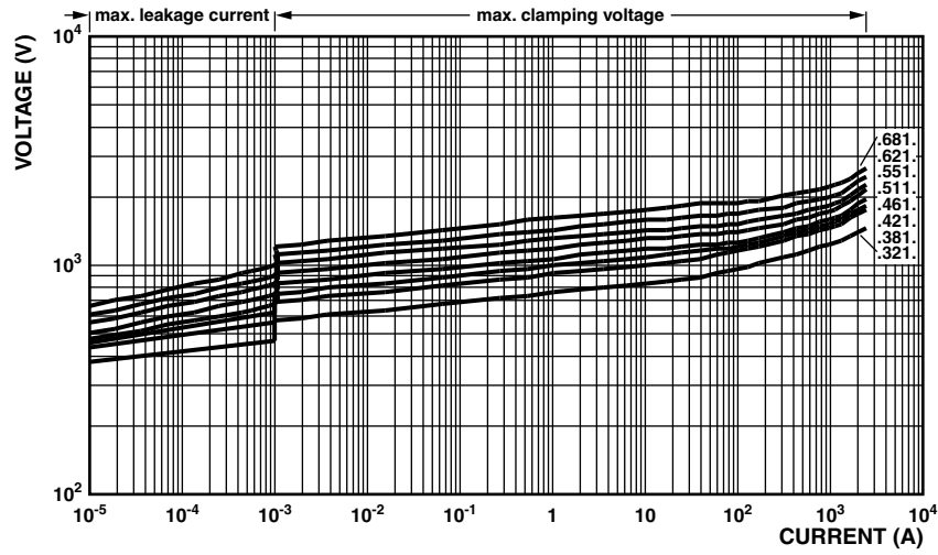
11 V RMS to 40 V RMS ; VDRH14.....E
