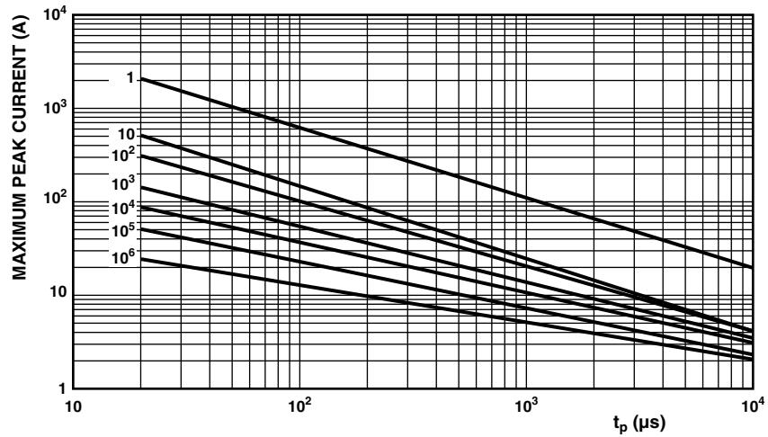
11 V RMS to 40 V RMS ; VDRH14.....E
