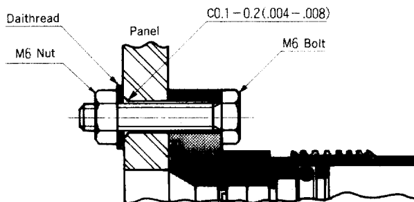
Mounting Method (2)
