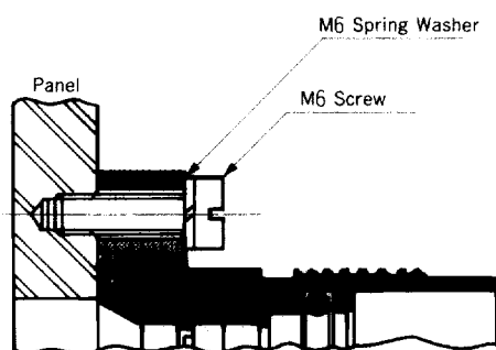
Mounting Method (1)
