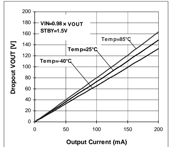
Figure 85. Dropout Voltage vs. Output Current
