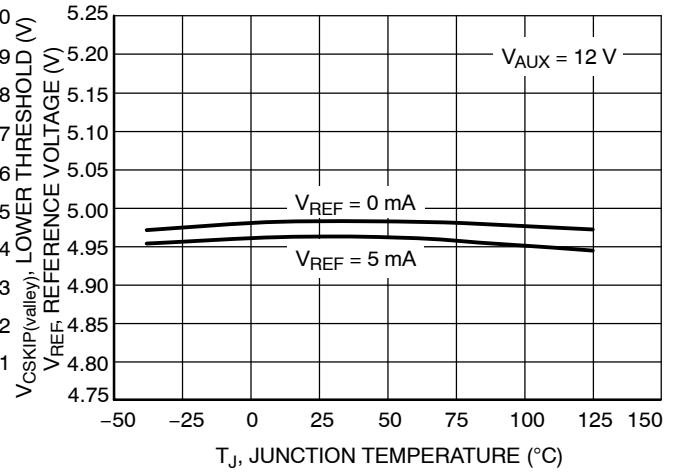
Figure 22. Reference Voltage vs. Junction Temperature
