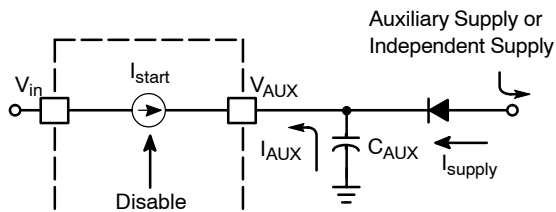
Figure 42. Recommended V_{AUX} Configuration
