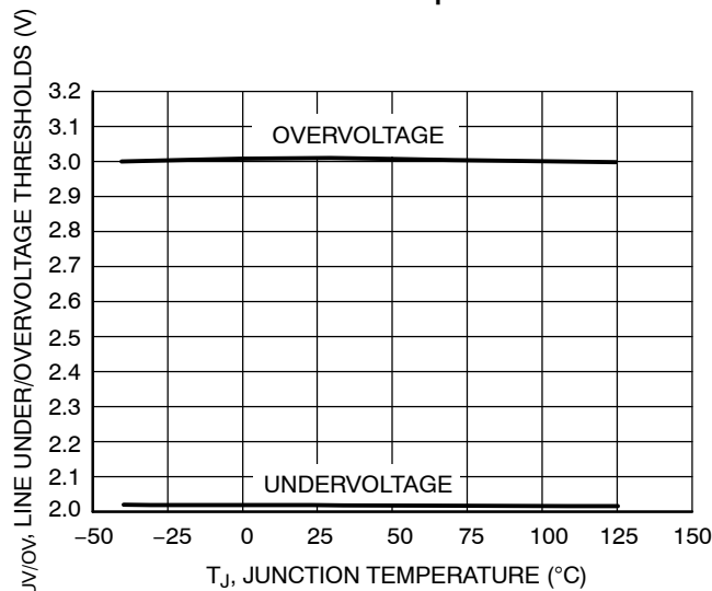
Figure 10. Line Under/Overvoltage Thresholds vs. Junction Temperature
