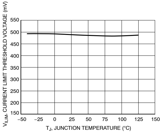
Figure 16. Current Limit Threshold Voltage vs. Junction Temperature
