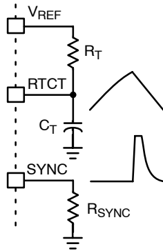
Figure 50. SYNC Pulse
