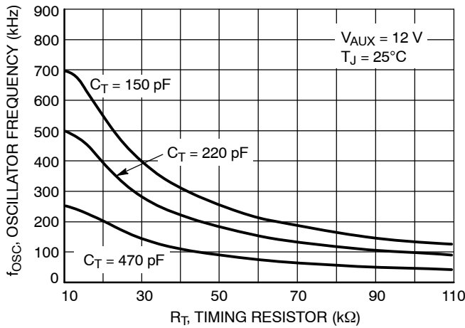
Figure 25. Oscillator Frequency vs. Timing Resistor
