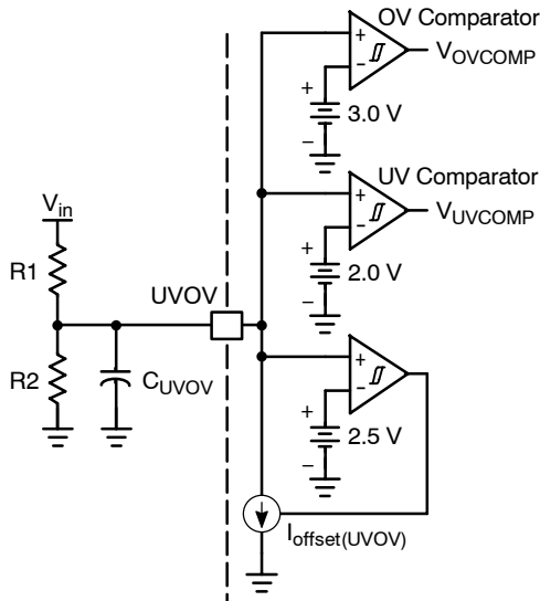
Figure 43. Line UVOV Detectors
