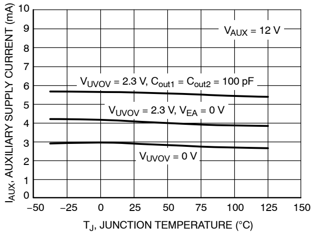
Figure 8. Auxiliary Supply Current vs. Junction Temperature
