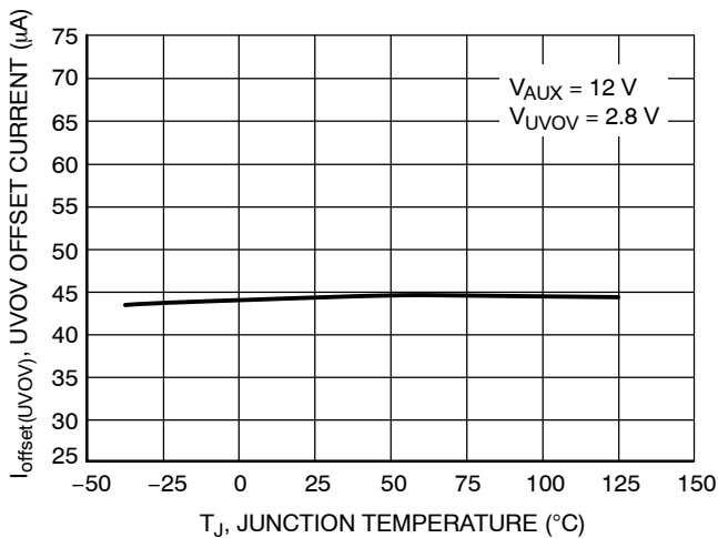
Figure 12. UV OV Offset Current vs. Junction Temperature
