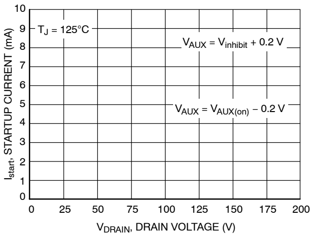
Figure 6. Startup Current vs. Drain Voltage
