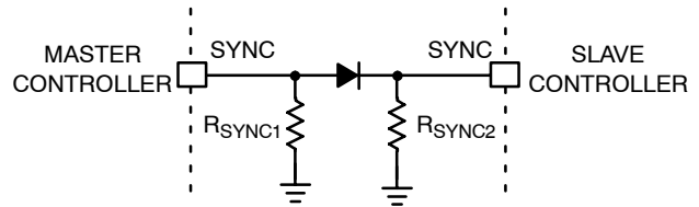
Figure 51. Master-Slave Configuration
