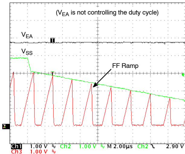
Figure 37. Soft-Stop Behavior After Soft-Start is Complete and V_{EA} is Open.
