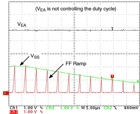
Figure 35. Soft-Stop Before Soft-Start is Complete and V_{\text{EA}} is Open.
