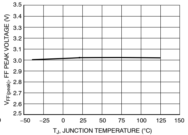
Figure 15. Feedforward Peak Voltage vs. Junction Temperature
