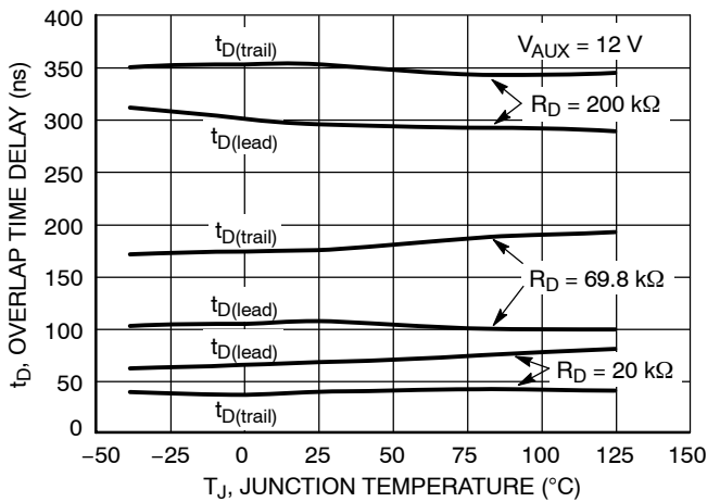
Figure 30. Overlap Time Delay vs. Junction Temperature
