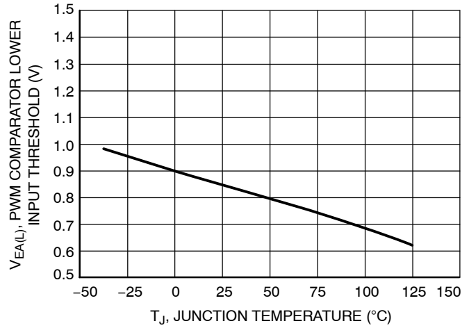
Figure 34. PWM Comparator Lower Input Threshold vs. Junction Temperature
