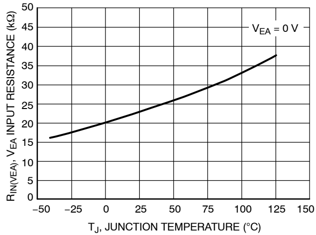
Figure 33. V EA Input Resistance vs. Junction Temperature
