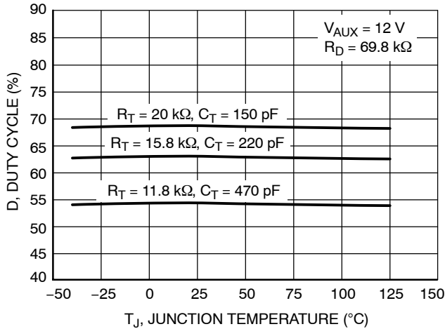
Figure 27. Duty Cycle vs. Junction Temperature
