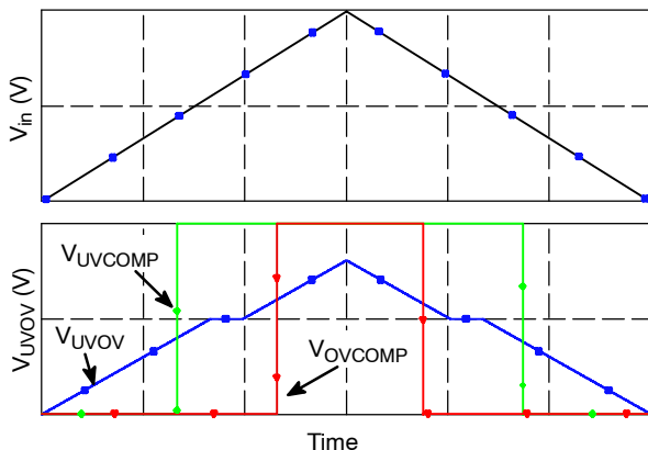
Figure 44. UVOV Detectors Typical Waveforms
