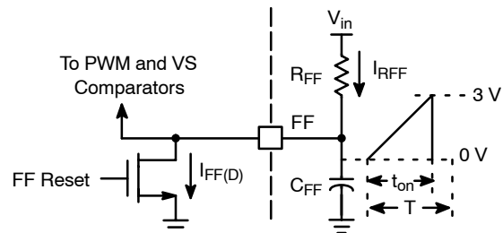
Figure 45. Feed Forward Ramp Generation
