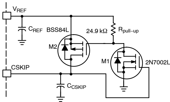
Figure 40. External Latch Implemented using Discrete N and P-Channel MOSFETs
