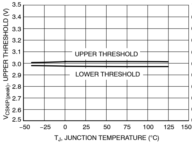
Figure 21. Cycle Skip Voltage Thresholds vs. Junction Temperature
