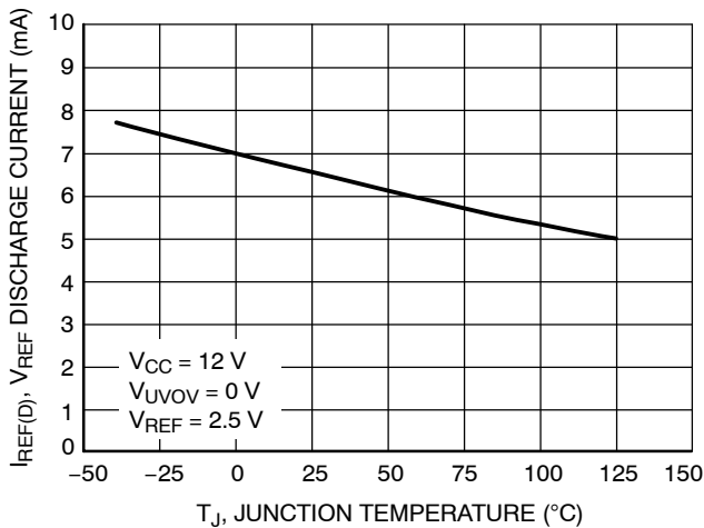
Figure 23. V_{REF} Discharge Current vs. Junction Temperature
