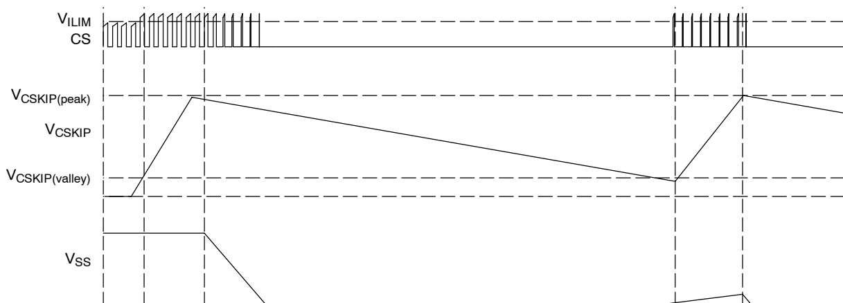
Figure 38. Cycle Skip Waveforms
