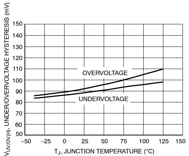
Figure 11. Line Under/Overvoltage Hysteresis vs. Junction Temperature
