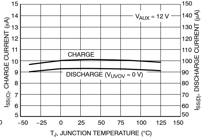
Figure 28. Soft-Start/Stop Charge and Discharge Currents vs. Junction Temperature
