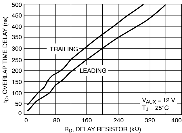
Figure 29. Overlap Time Delay vs. Delay Resistor
