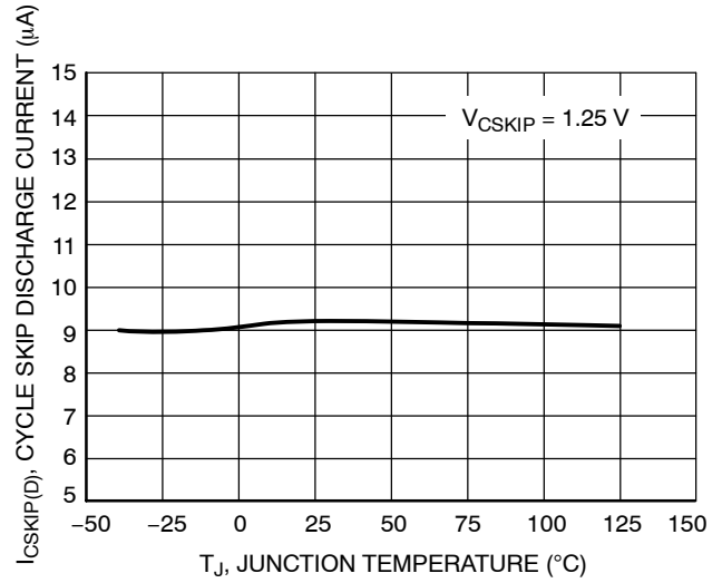
Figure 20. Cycle Skip Discharge Current vs. Junction Temperature
