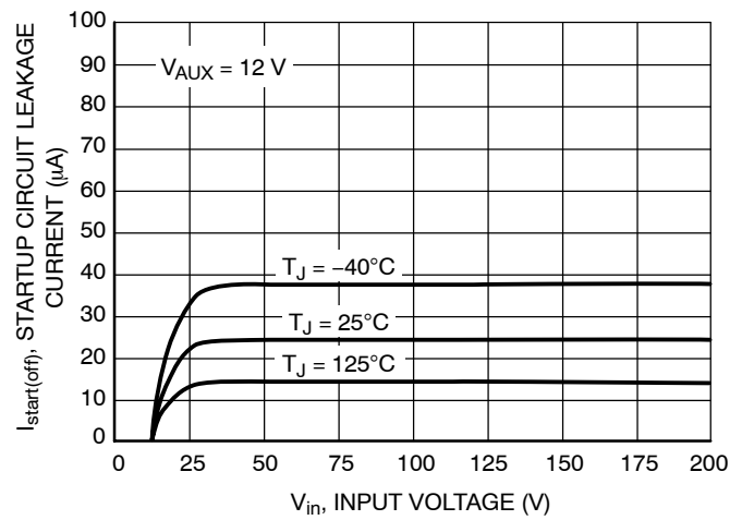
Figure 7. Startup Circuit Leakage Current vs. Input Voltage
