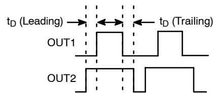
Figure 48. Output Timing Diagram
