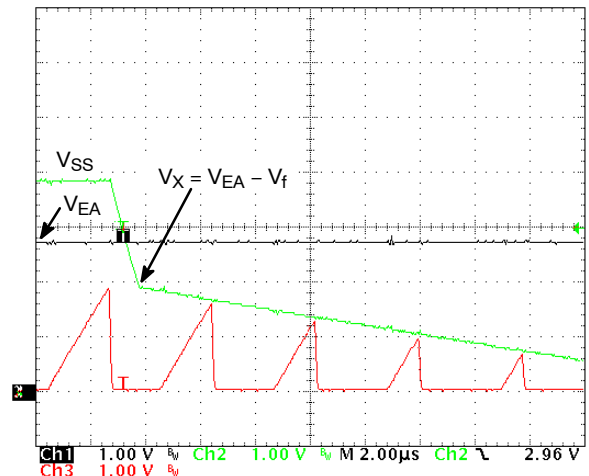
Figure 36. Soft-Stop Behavior when V_{\text{EA}} Controls the Duty Cycle.
