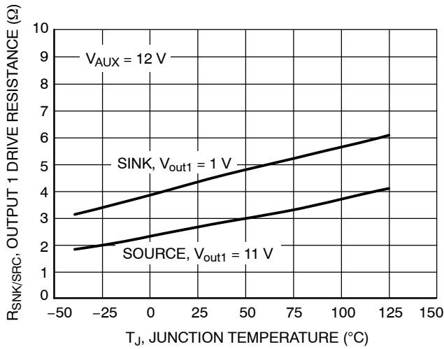
Figure 31. Output 1 Drive Resistance vs. Junction Temperature
