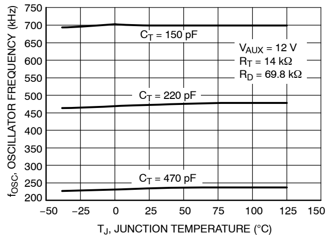
Figure 24. Oscillator Frequency vs. Junction Temperature
