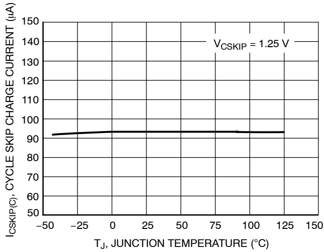
Figure 19. Cycle Skip Charge Current vs. Junction Temperature
