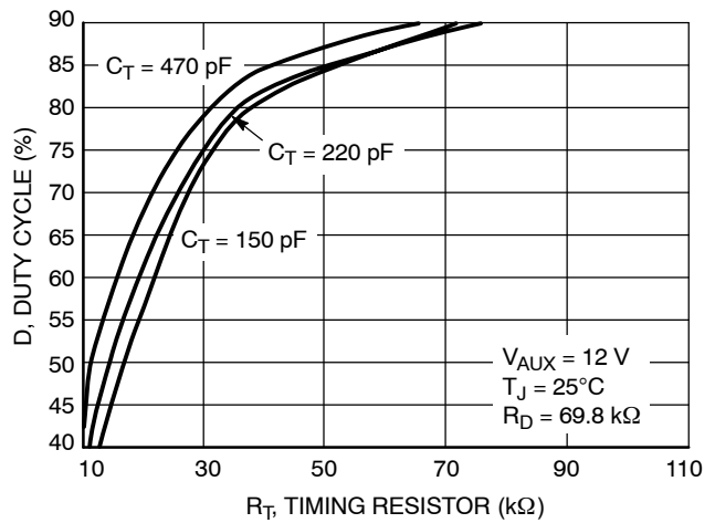
Figure 26. Duty Cycle vs. Timing Resistor
