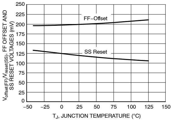
Figure 14. FF Offset and SS Reset Voltages vs. Junction Temperature
