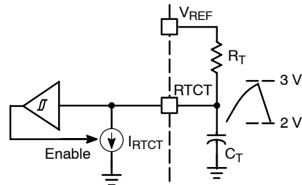
Figure 49. Oscillator Configuration
