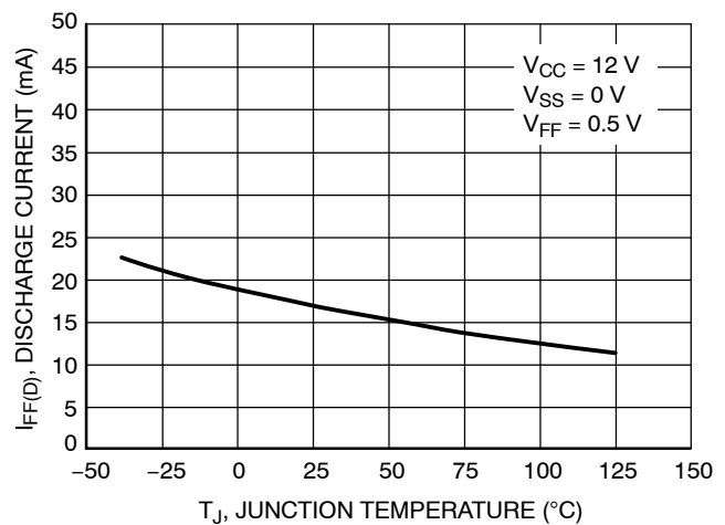
Figure 13. FF Discharge Current vs. Junction Temperature
