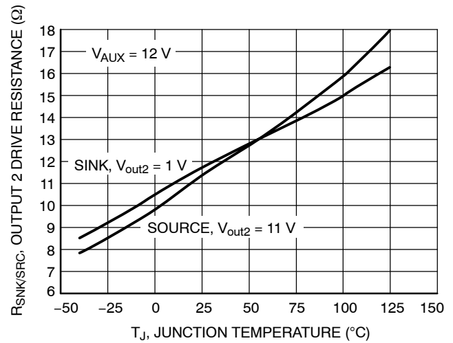
Figure 32. Output 2 Drive Resistance vs. Junction Temperature
