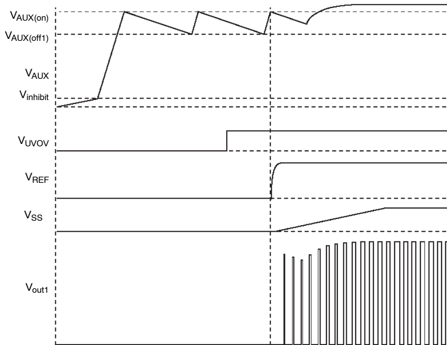
Figure 41. Startup Circuit Waveforms
