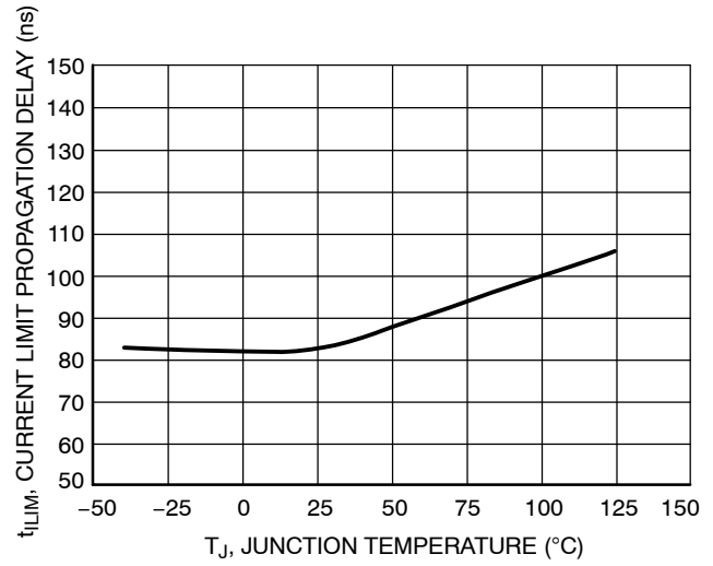
Figure 17. Current Limit Propagation Delay vs. Junction Temperature
