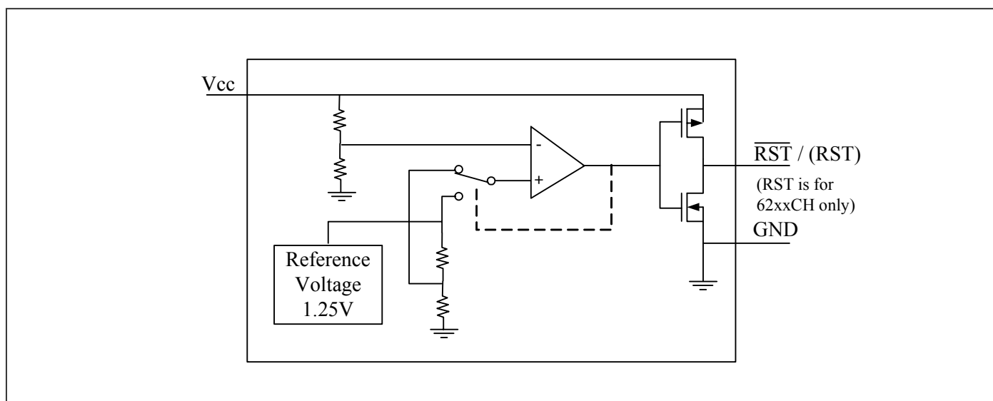
Block Diagram of PT7M62xxCL/CH/CLL
