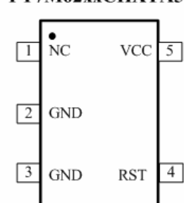
PT7M62xxCHXTA5
