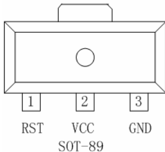
PT7M62xxCHXTD
