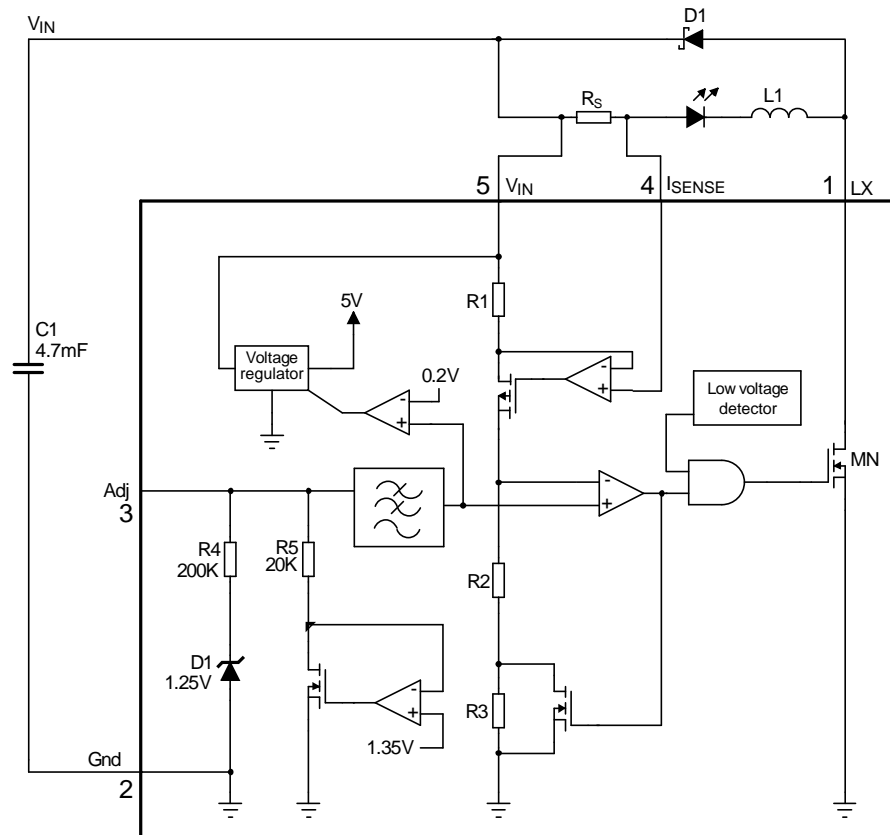
Figure 1. Block diagram – Pin Connection for TSOT23-5 Package
