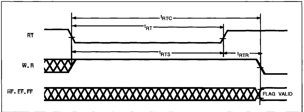
Figure 11 : Retransmit.
