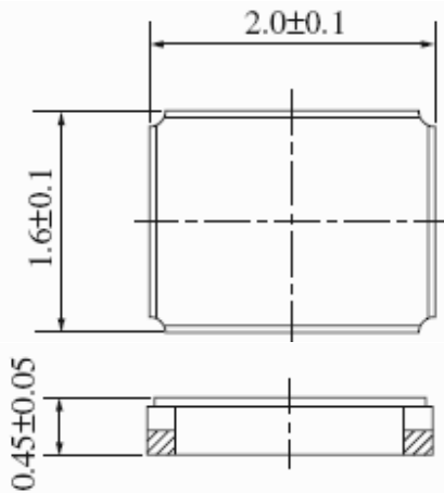
Figure 1) Top, Side and End Views
