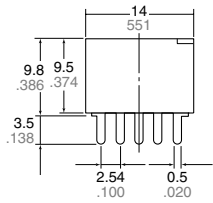
External dimensions Standard PC board terminal
