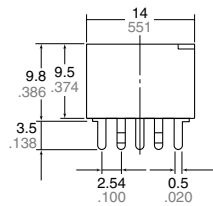
Self-clinching terminal
