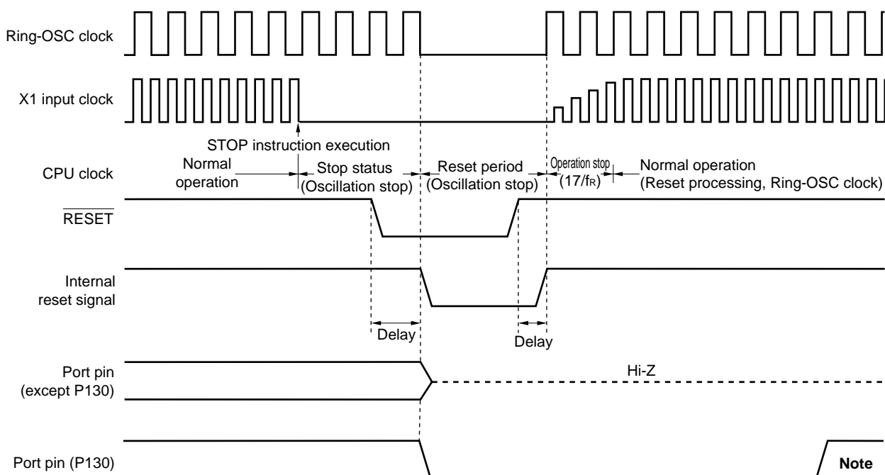
Figure 16-4. Timing of Reset in STOP Mode by \overline{\text{RESET}} Input
