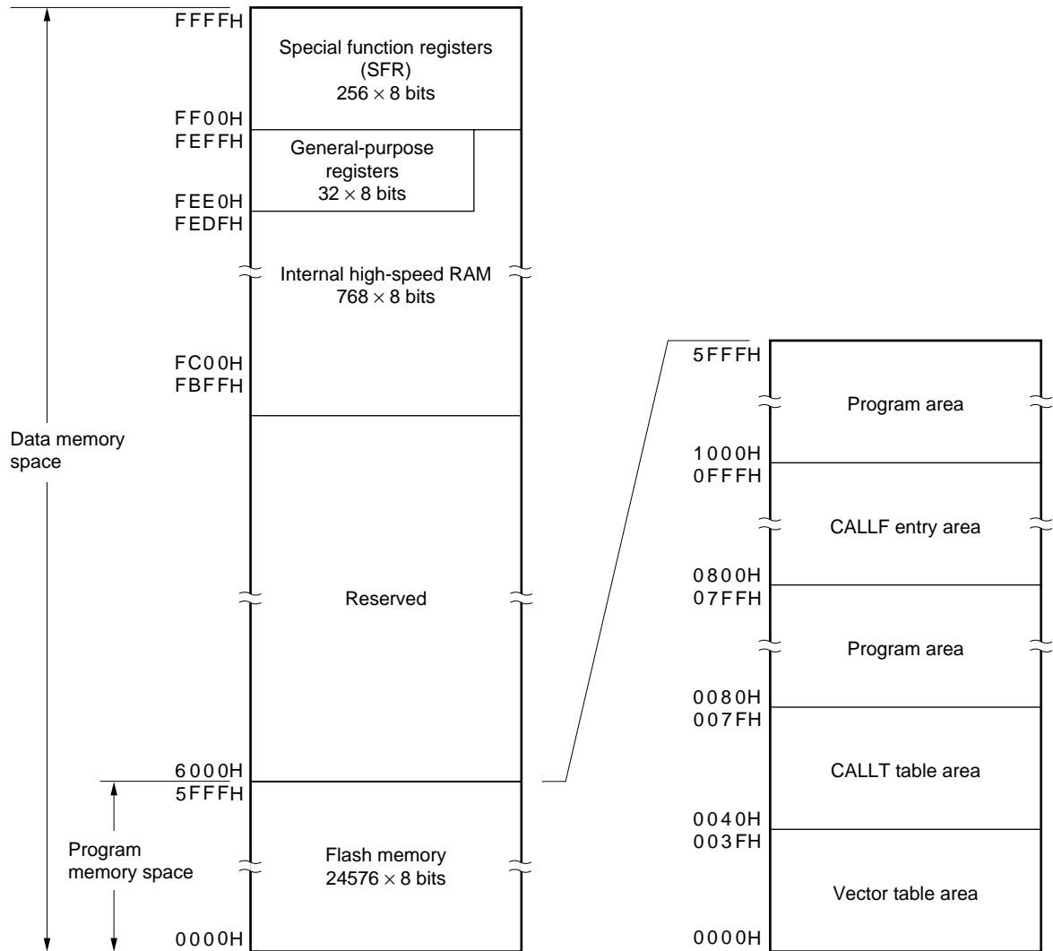
Figure 3-4. Memory Map ( \mu PD78F0103)
