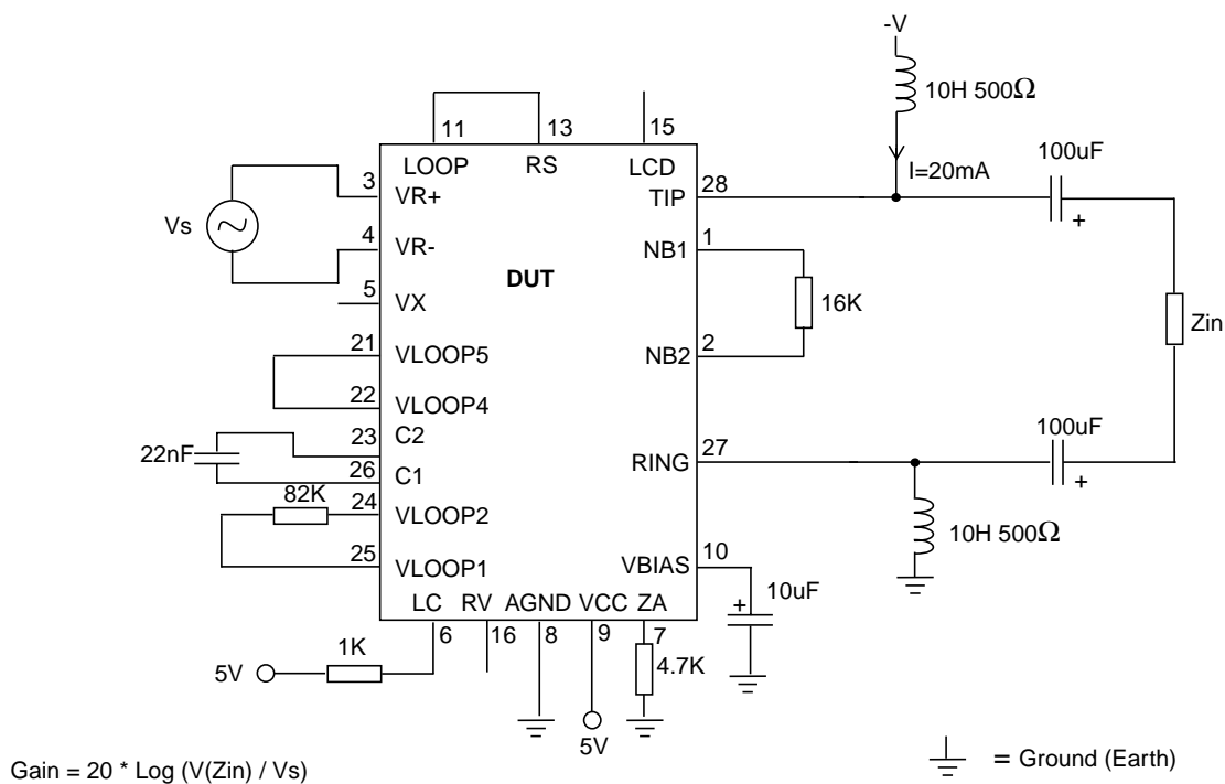
Figure 8 - Test Circuit 3
