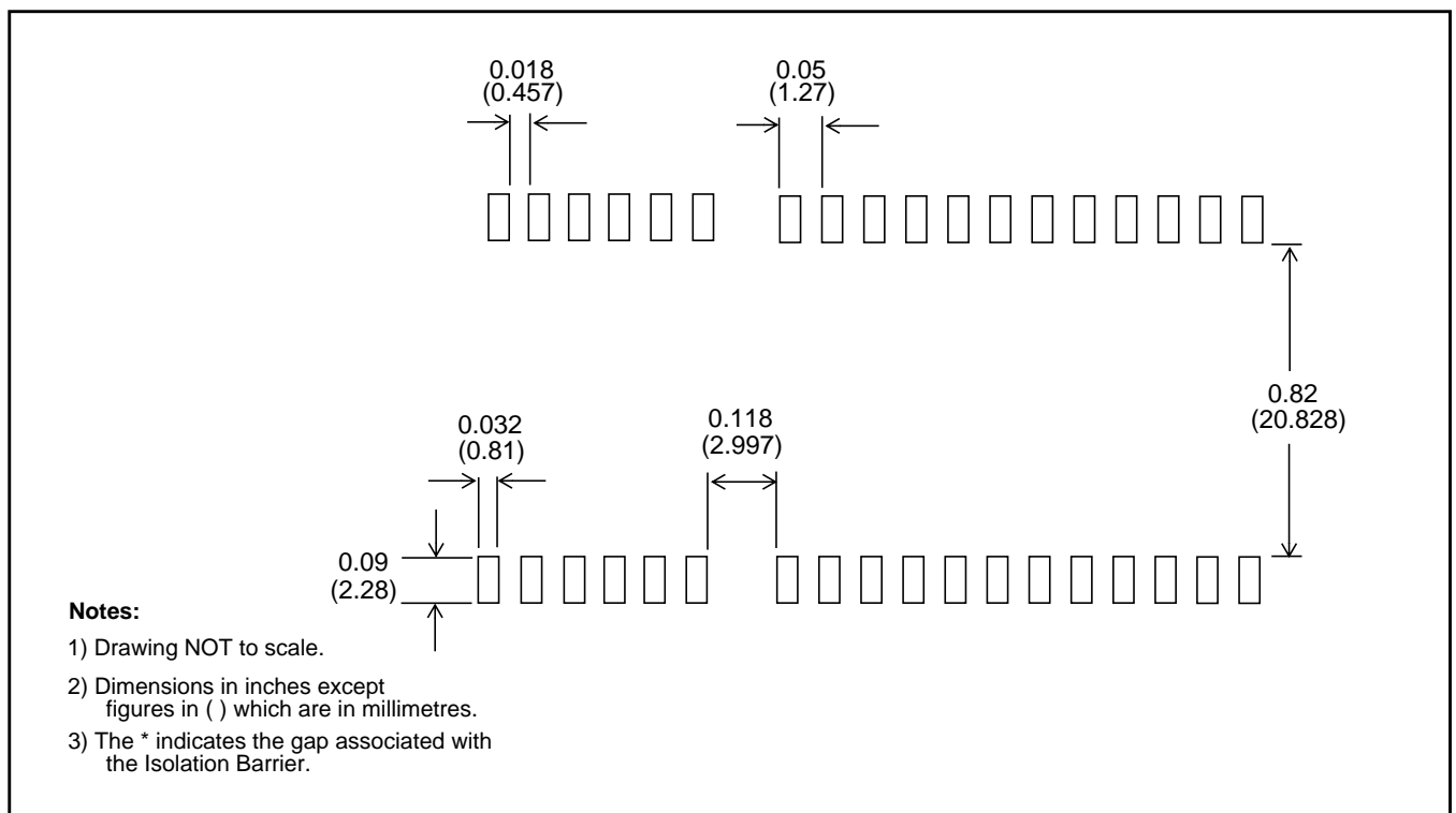
Figure 15 - Recommended Footprint for AF-P Package Device
