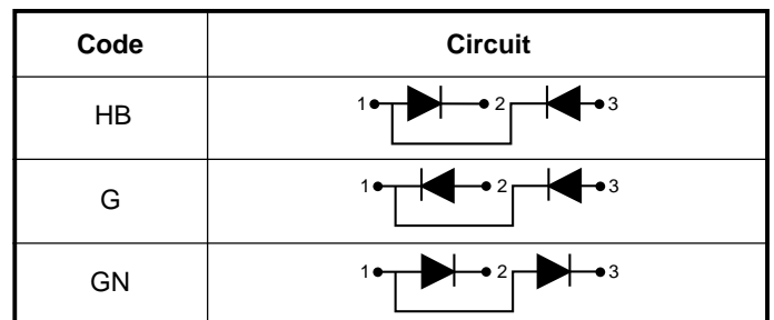
Fig.1 Circuit diagrams
