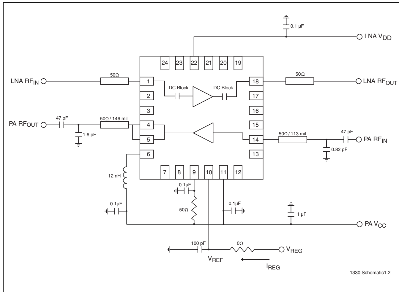
FIGURE 15: Typical Schematic
