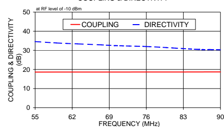
ZDC-20-3-75-1 COUPLING & DIRECTIVITY
